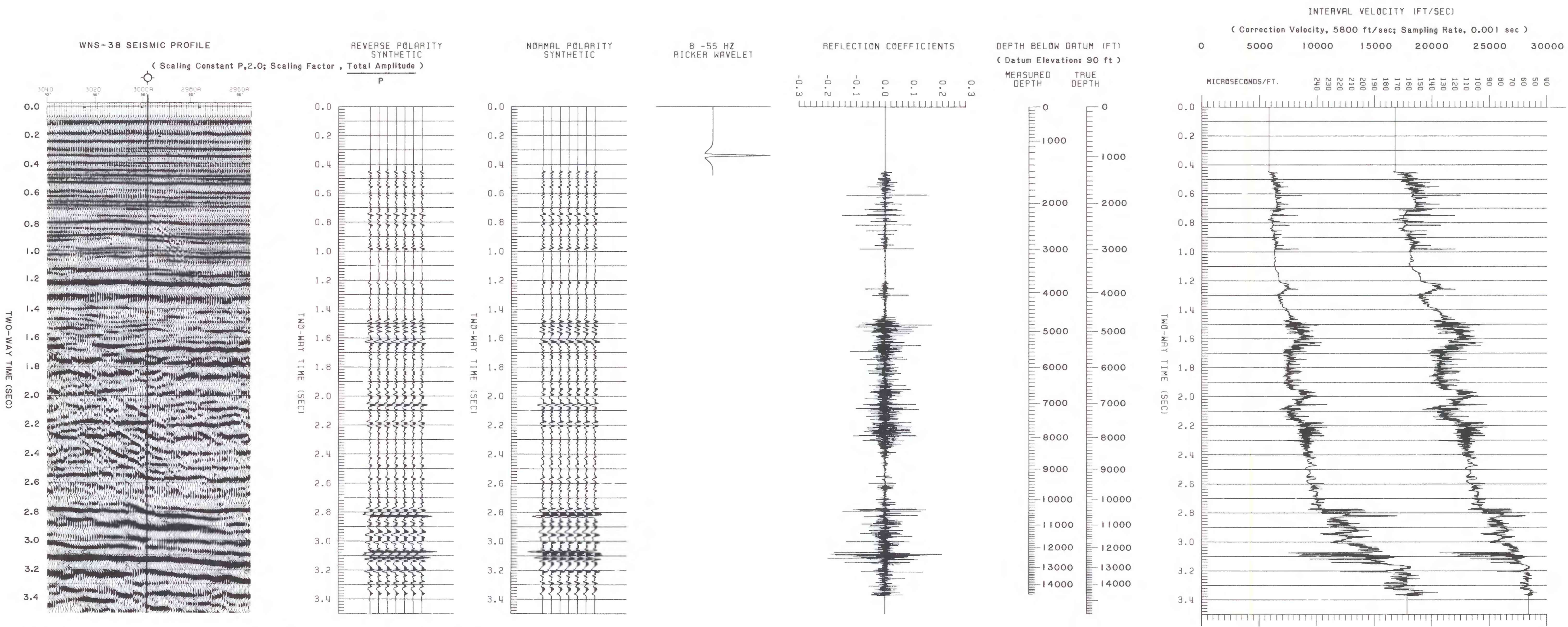
FIGURE 7. Synthetic Seismogram of ARCO's Norton Sound COST No. 1 Well.
