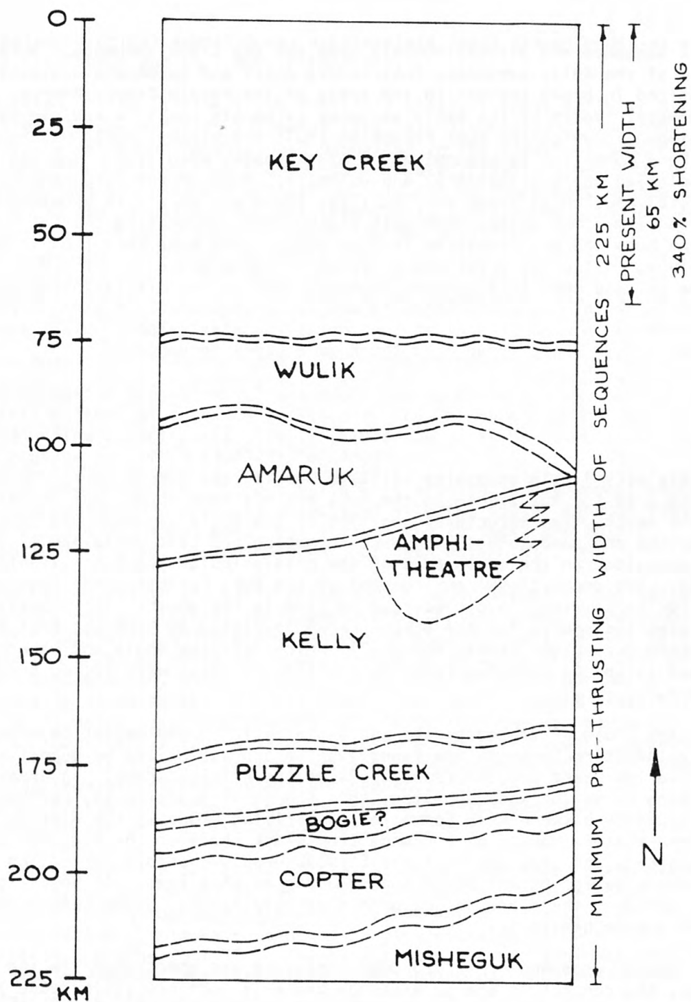
Figure 5.--Generalized palinspastic map of sequences exposed in the south central and southeastern De Long Mountains quadrangle, prior to Mesozoic thrust faulting. Inferred direction of thrust transport is along a north-south line. The width of sequences is based on outcrops within the map area only, and does not take into account extent of some sequences south of the De Long Mountains quadrangle. See text for more complete explanation.
