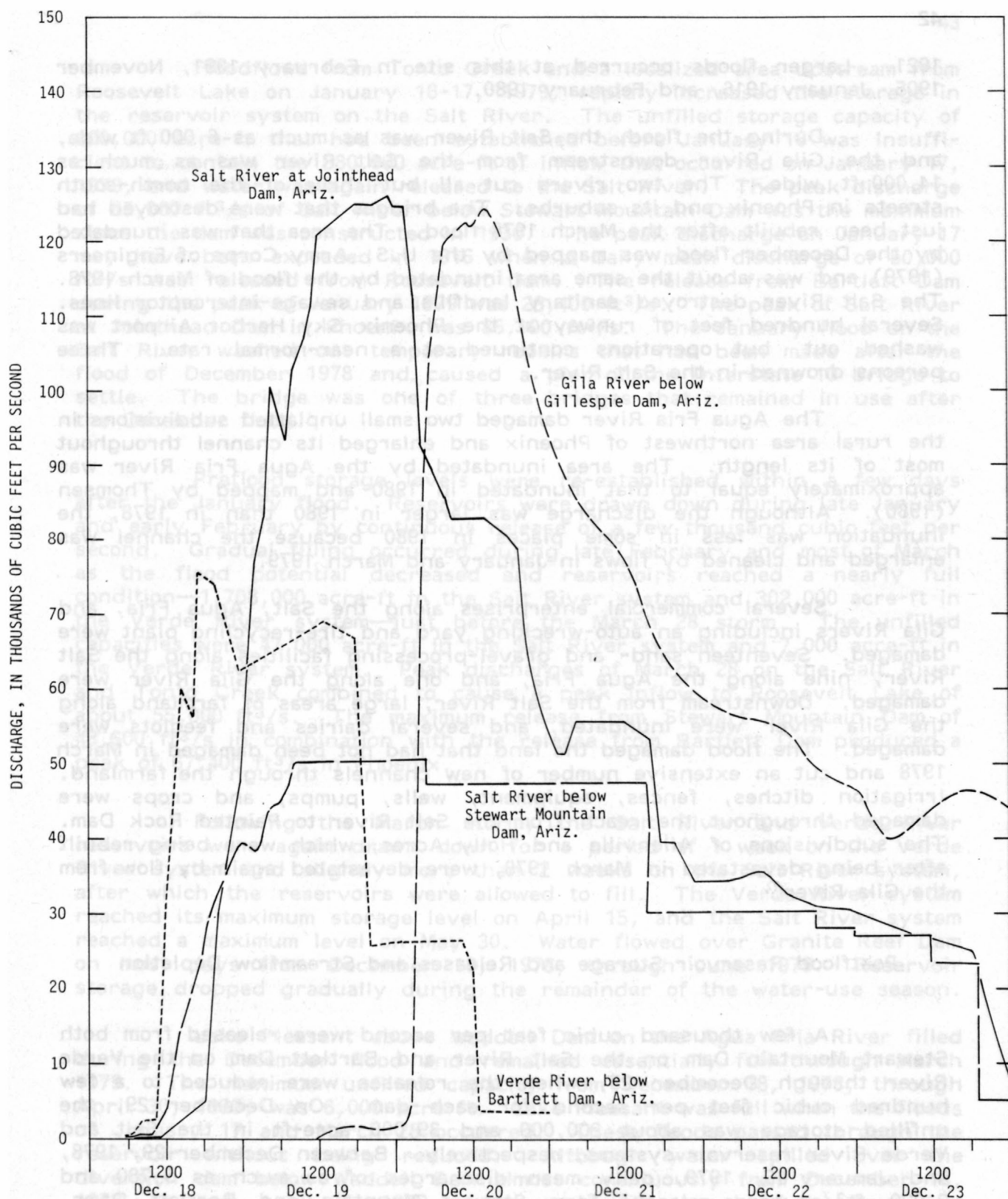
Figure 10.--Regulated discharge of Salt, Verde, and Gila Rivers, December 18-23, 1978.
