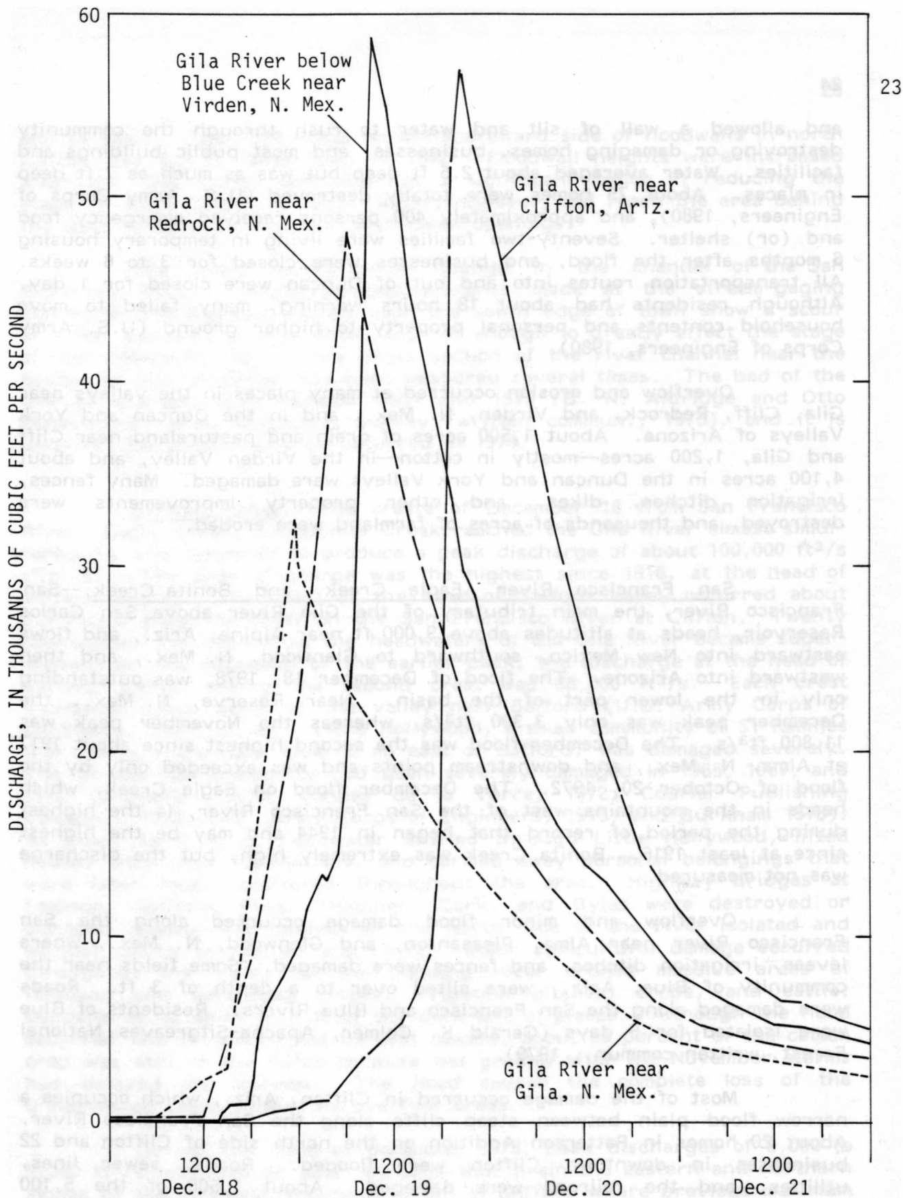
Figure 5.--Discharge of the Gila River at gaging stations upstream from San Francisco River in Arizona and New Mexico, December 18-21, 1978.
