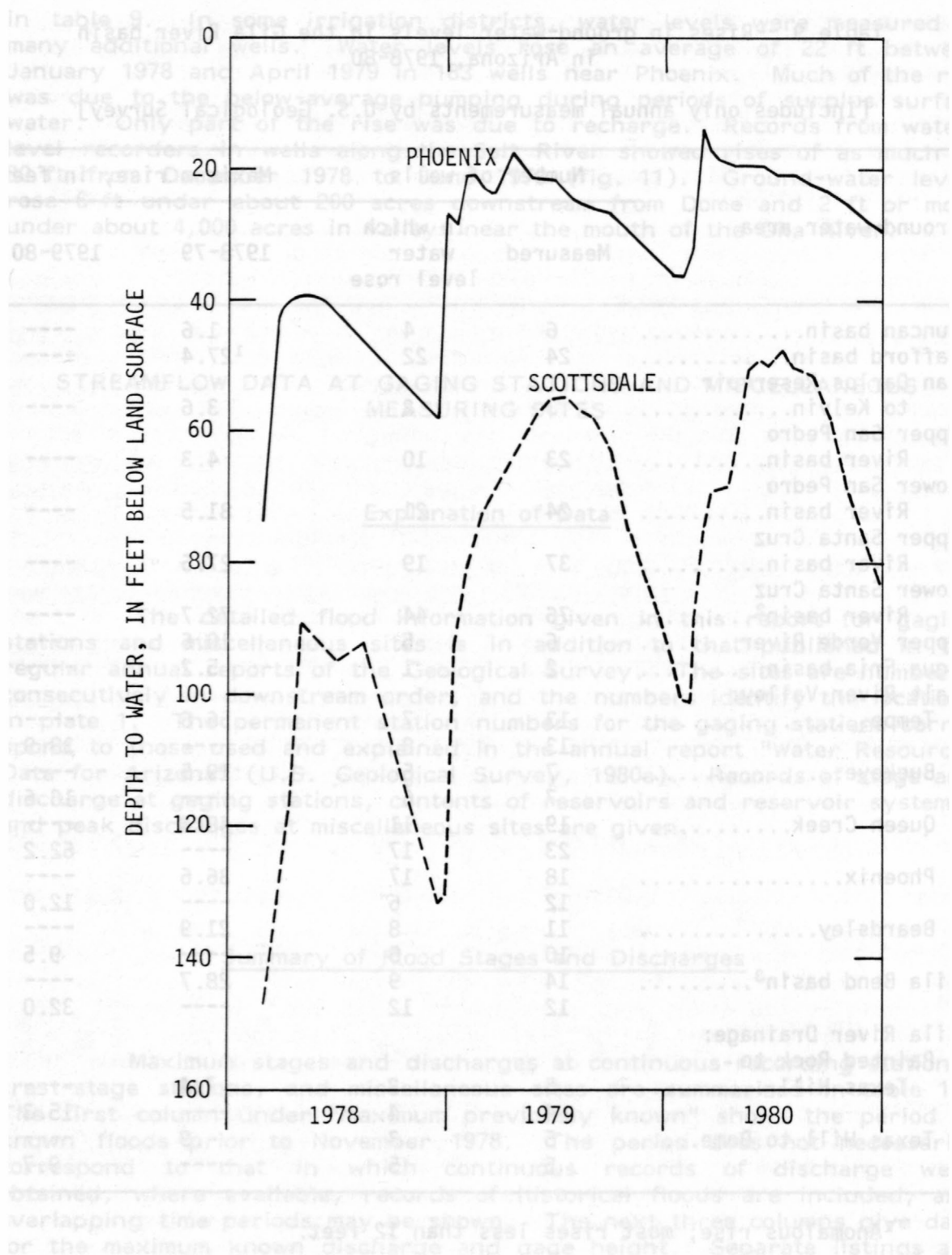
Figure 11.--Depth to water recorded in wells near the Salt River at Phoenix and Scottsdale, Ariz., 1978-80.
