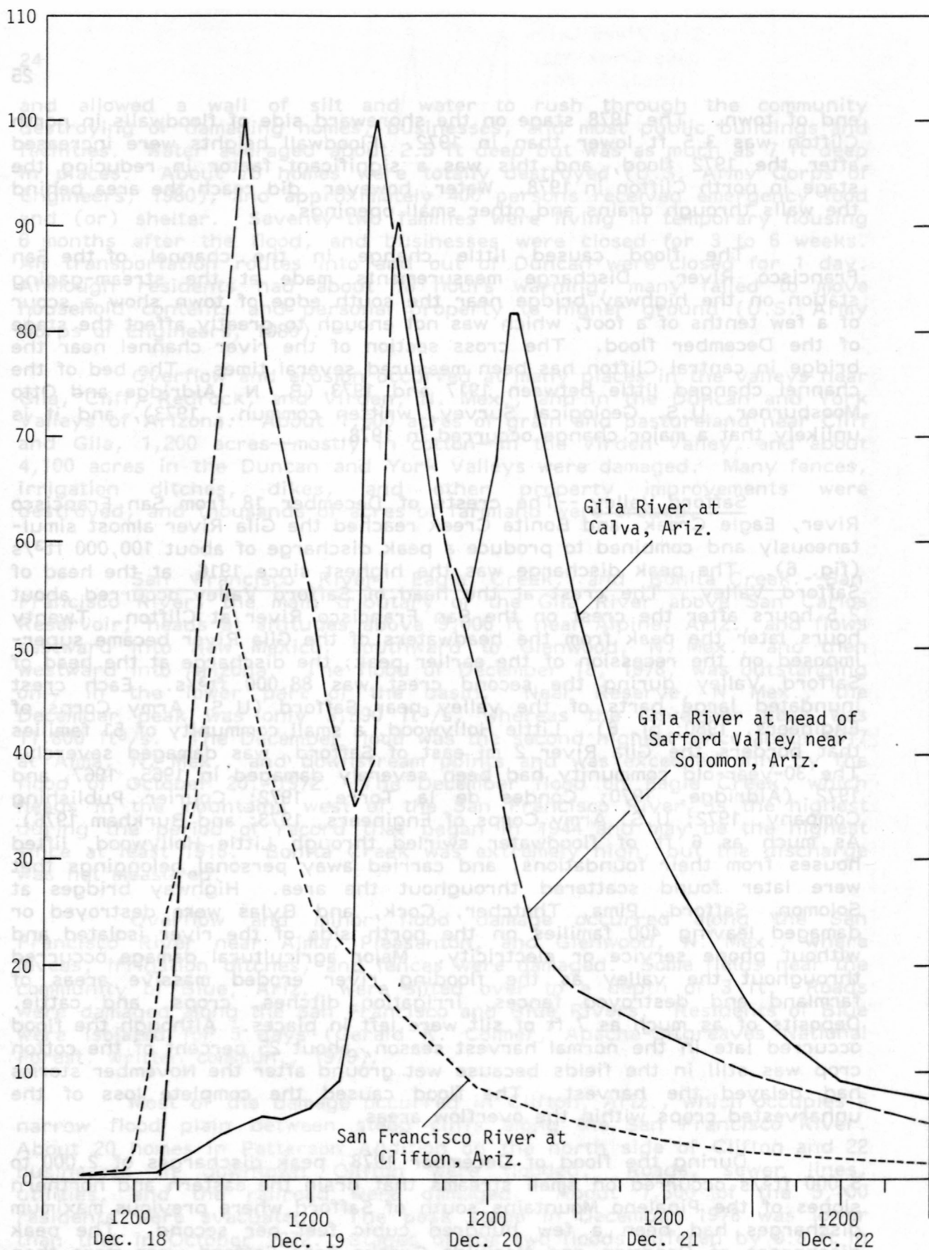
Figure 6.--Discharge of the San Francisco River at Clifton and Gila River at gaging stations between San Francisco River and San Carlos Reservoir, December 18-22, 1978.
