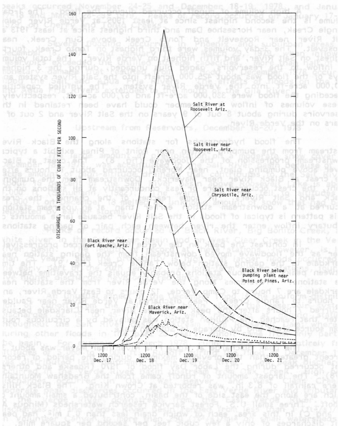
Figure 8.--Discharge at gaging stations on the Black and Salt Rivers upstream from Roosevelt Lake, Ariz., December 17-21, 1978.
