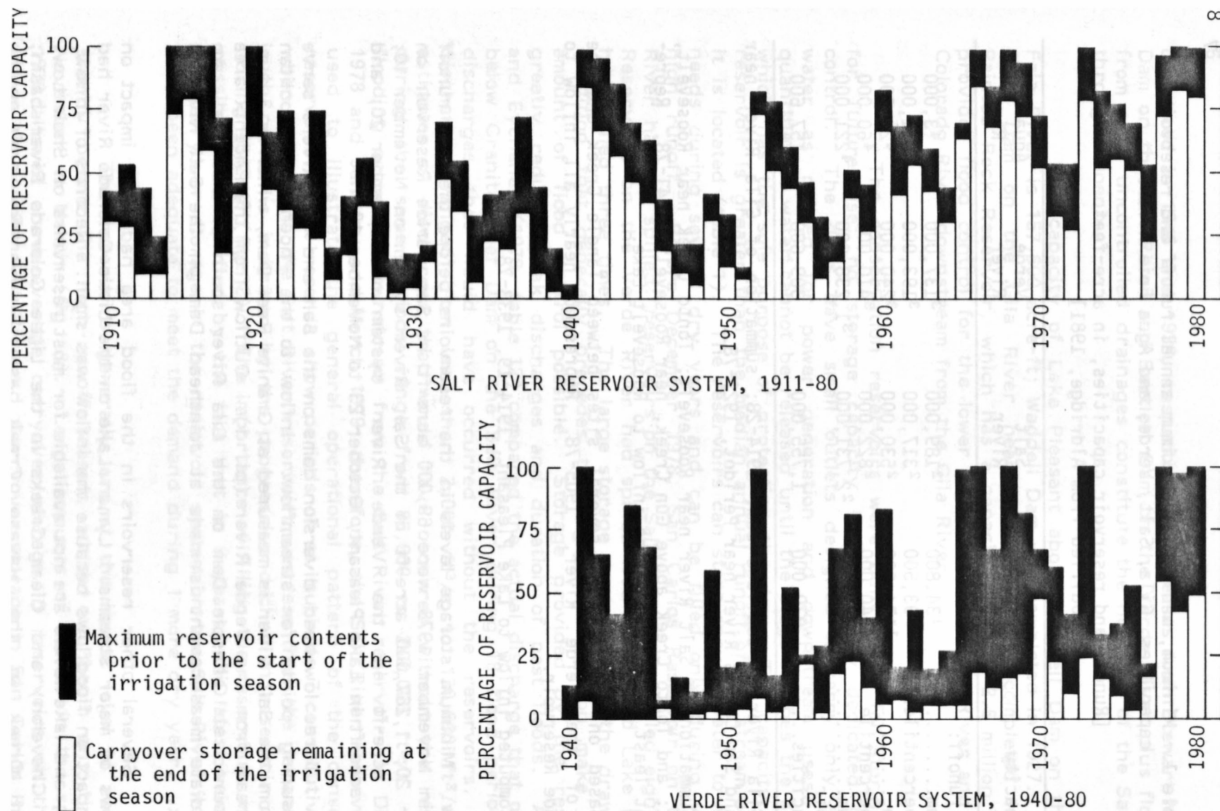
Figure 2.--Maximum reservoir contents and carryover storage, Salt River reservoir system, 1911-80, and Verde River reservoir system, 1940-80 (Aldridge, 1981).
