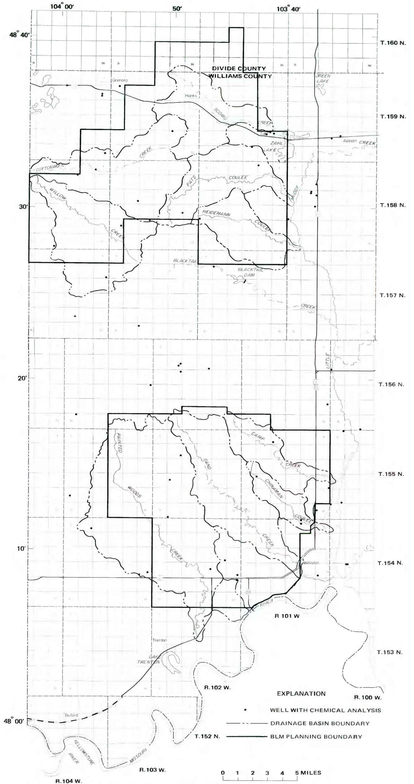
FIGURE 5.— Location of wells with chemical analyses in the Sand Creek-Hanks coal area.
