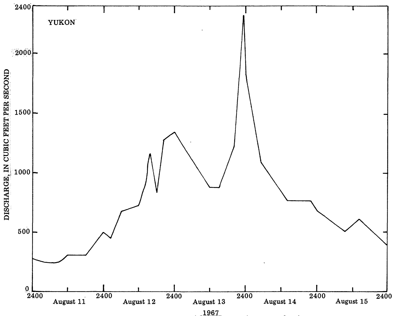
Figure 10. -- Discharge for Phelan Creek near Paxson.
