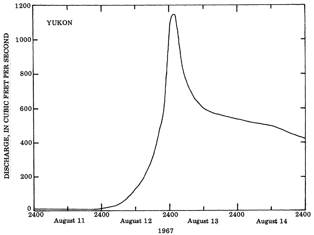
Figure 7. -- Discharge for Boulder Creek near Central.
