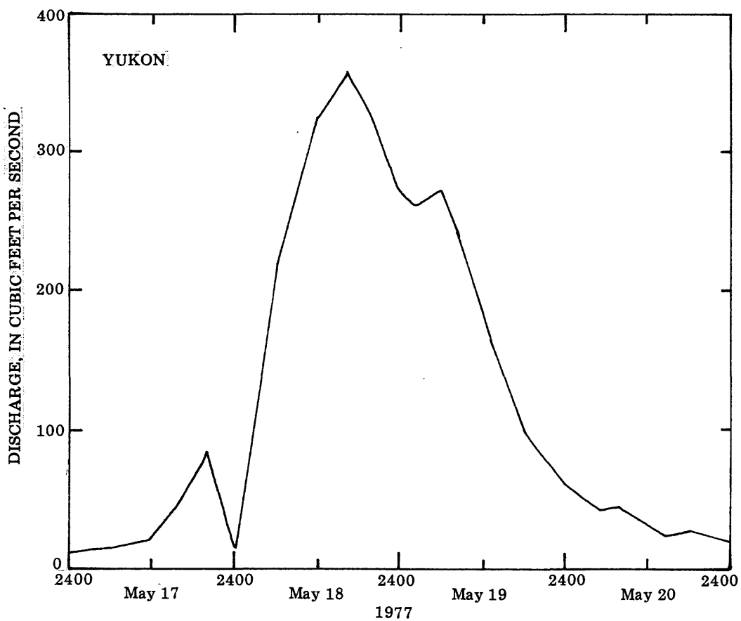
Figure 12. -- Discharge for Ophir Creek near Takotna.
