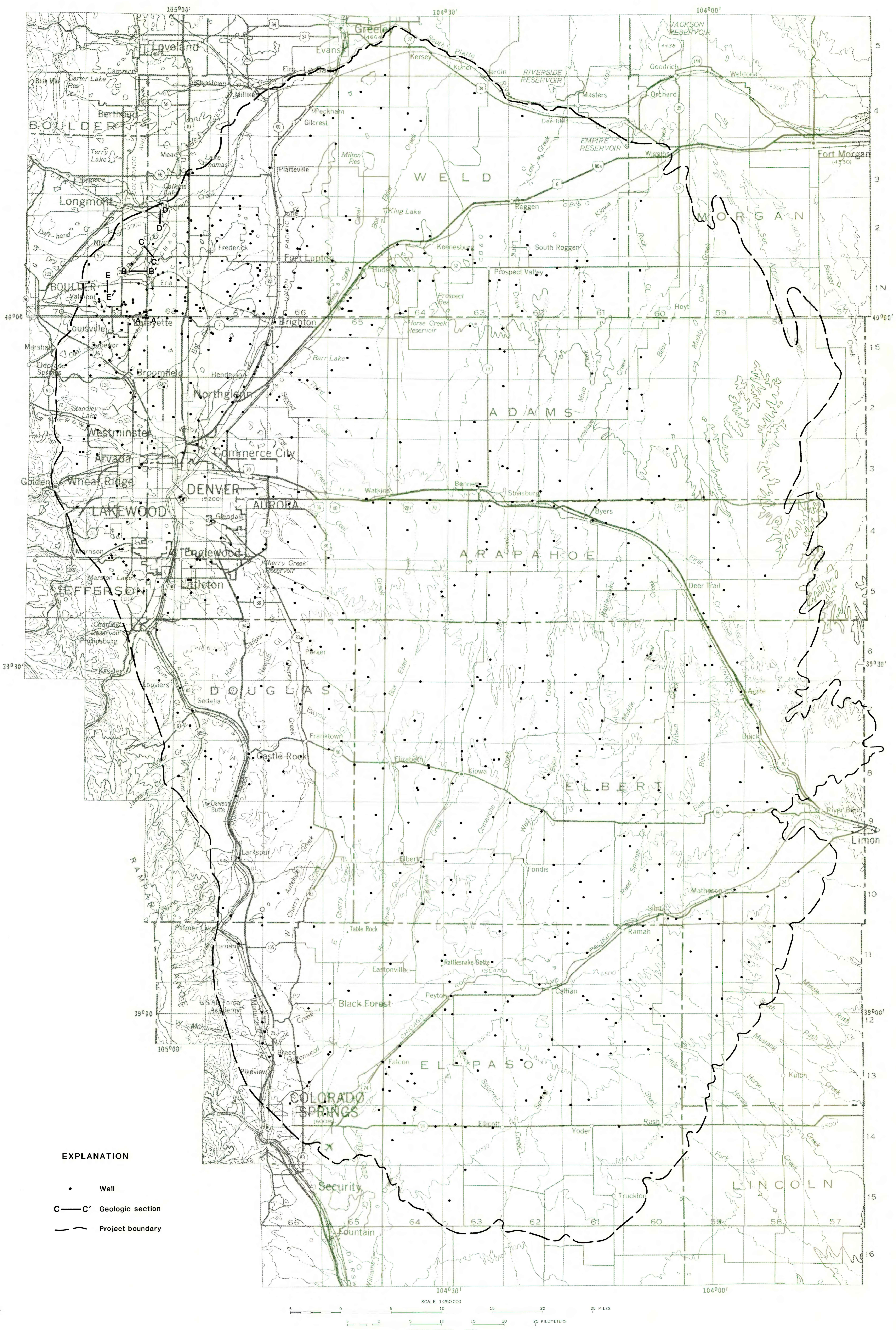
LOCATION OF SELECTED WELLS AND GEOLOGIC SECTIONS IN THE DENVER BASIN, COLORADO.
