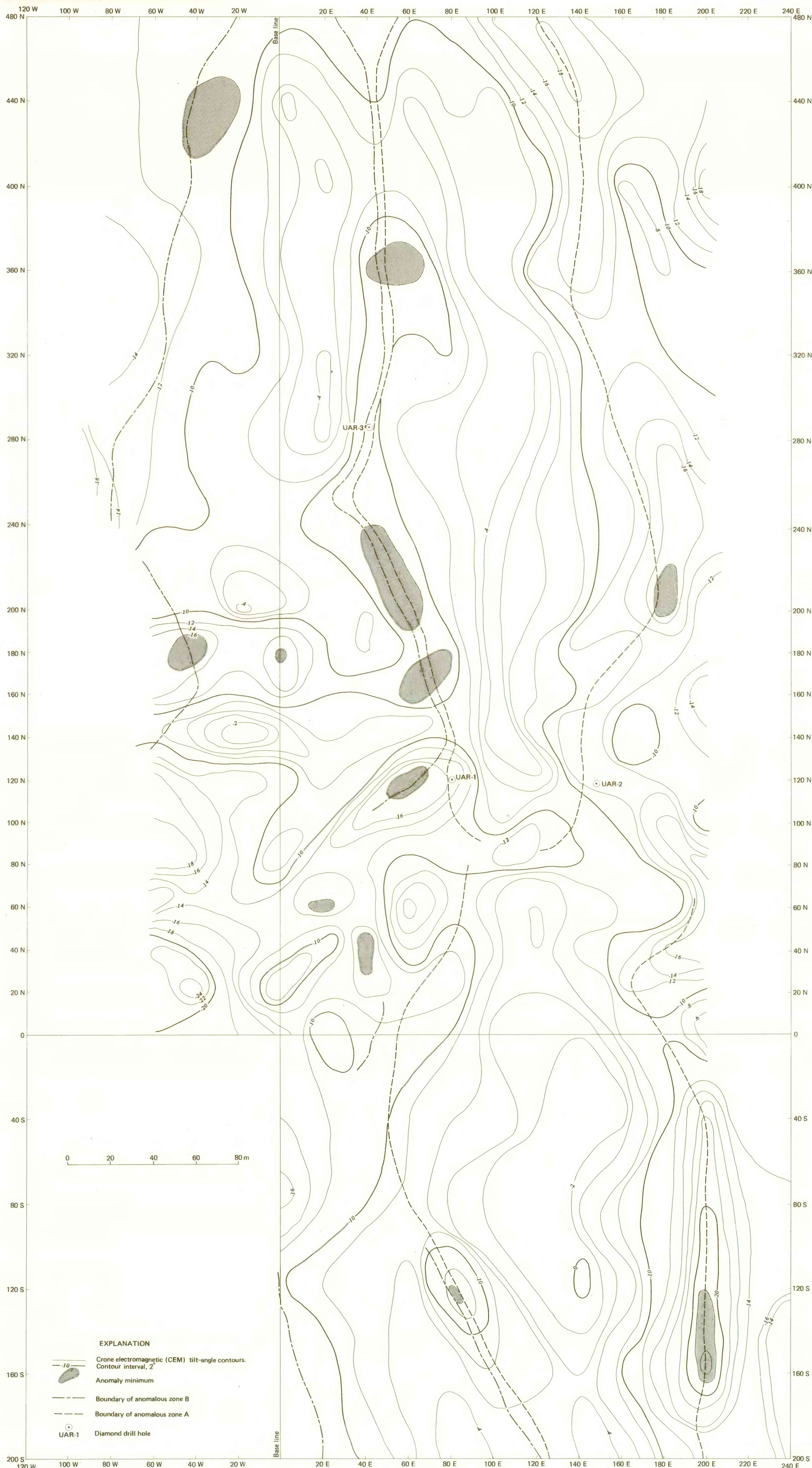
CRONE ELECTROMAGNETIC (CEM) TILT-ANGLE CONTOUR MAP, 5010 HZ, UMM AR RUMMF PROSPECT, KINGDOM OF SAUDI ARABIA
