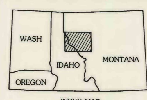
MAP SHOWING GEOLOGY AND SAMPLE LOCALITIES AND CONCENTRATION OF LEAD IN NONMAGNETIC HEAVY-MINERAL CONCENTRATES FROM THE WALLACE 1° x 2° QUADRANGLE, MONTANA AND IDAHO
