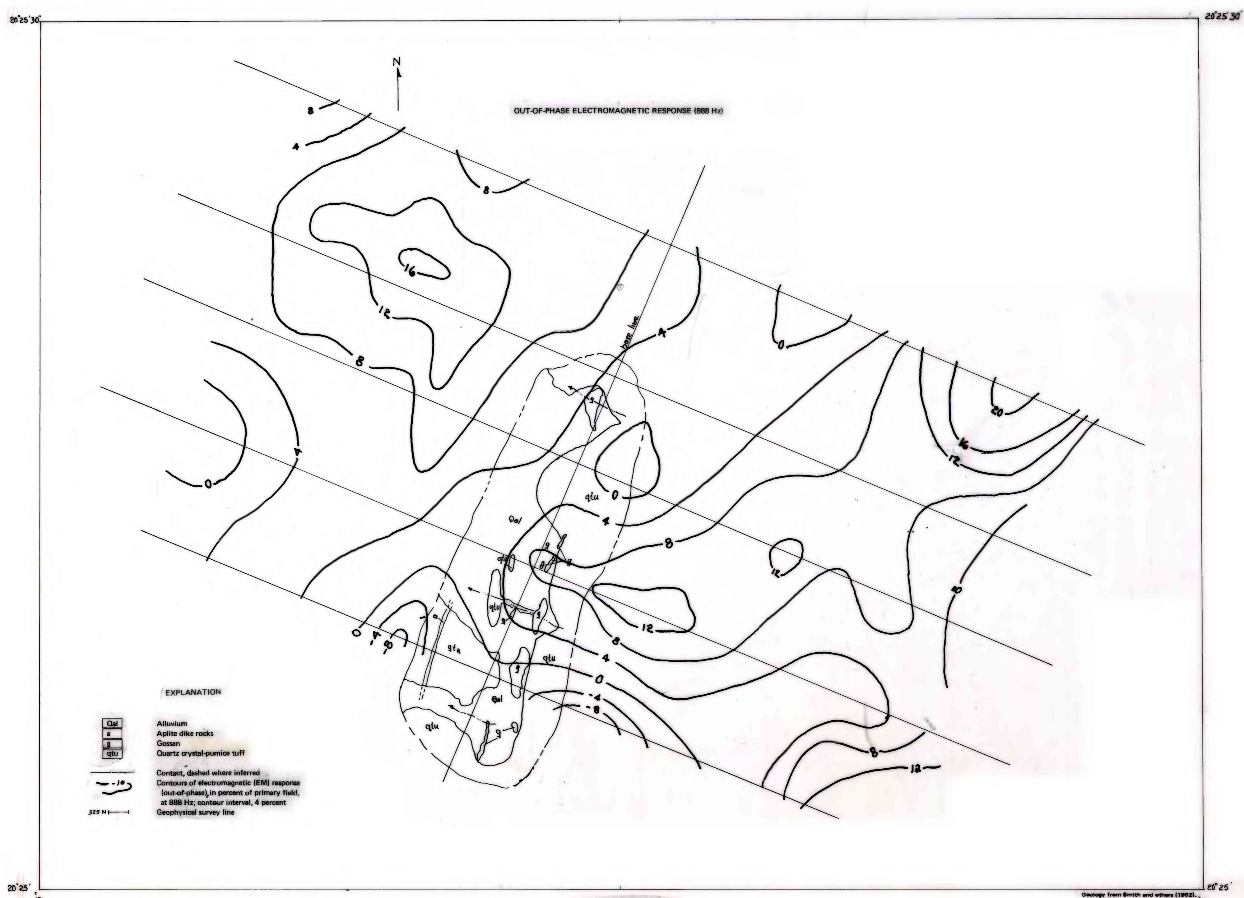
MAPS SHOWING SELF-POTENTIAL RESPONSE, AND IN-PHASE AND OUT-OF-PHASE ELECTROMAGNETIC RESPONSE (888 Hz), MULHAL No. 2 AREA, WADI BIDAH DISTRICT, KINGDOM OF SAUDI ARABIA
