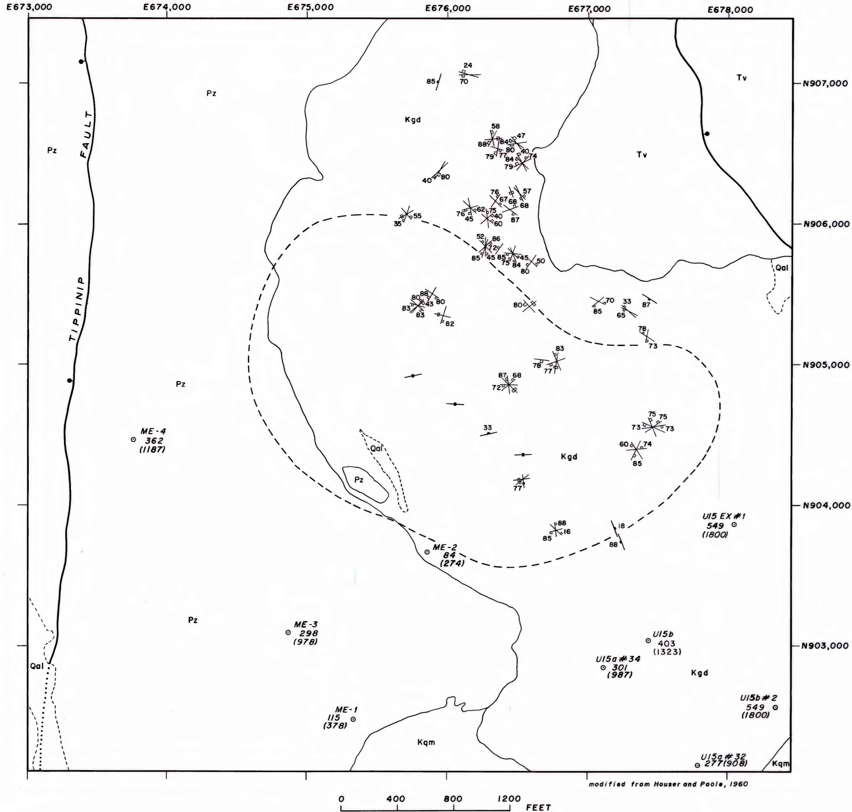
Geologic map of area of proposed emplacement holes
