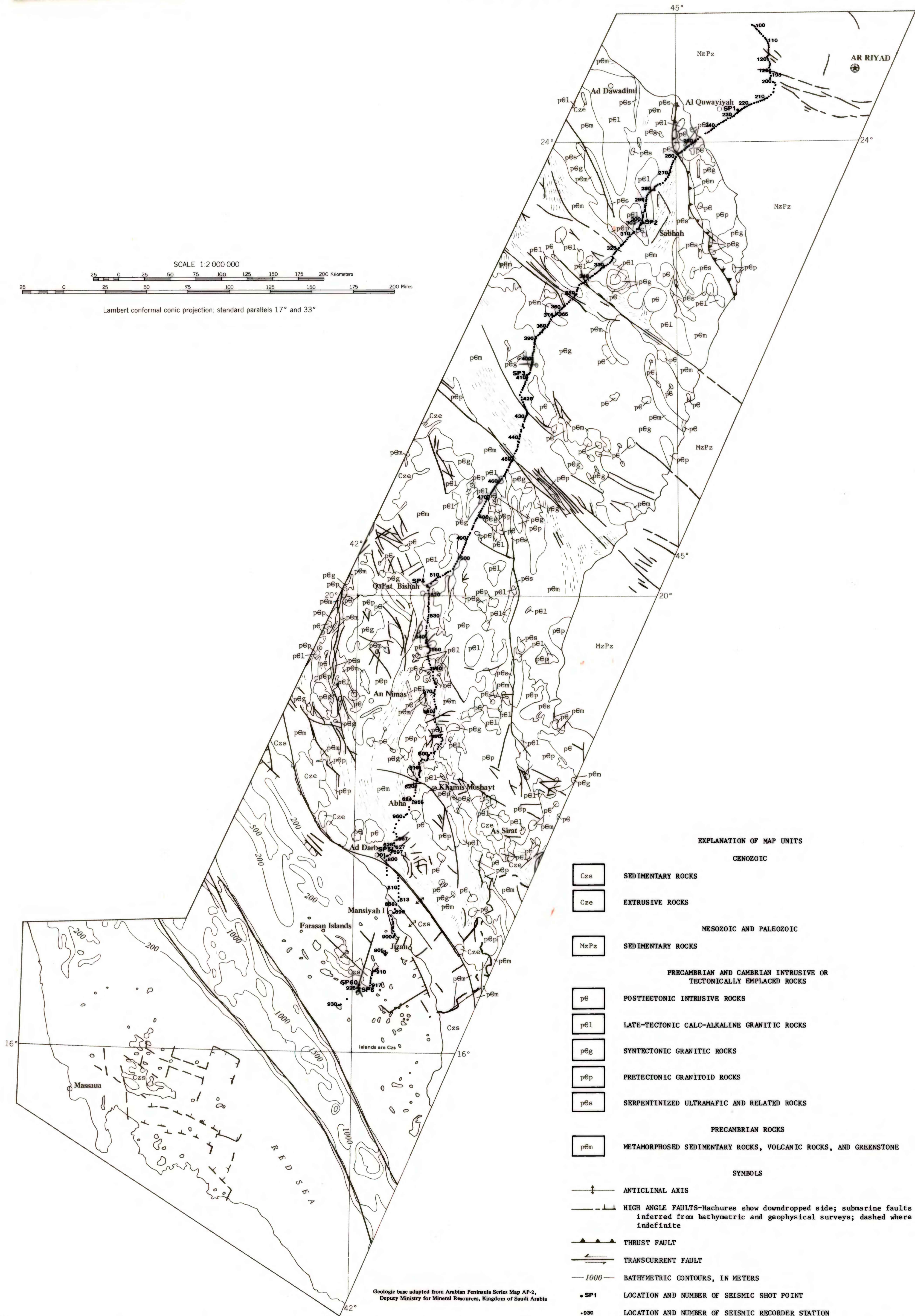
TECTONIC MAP OF PART OF WESTERN SAUDI ARABIA SHOWING RECORDER LOCATIONS AND SHOT POINTS
