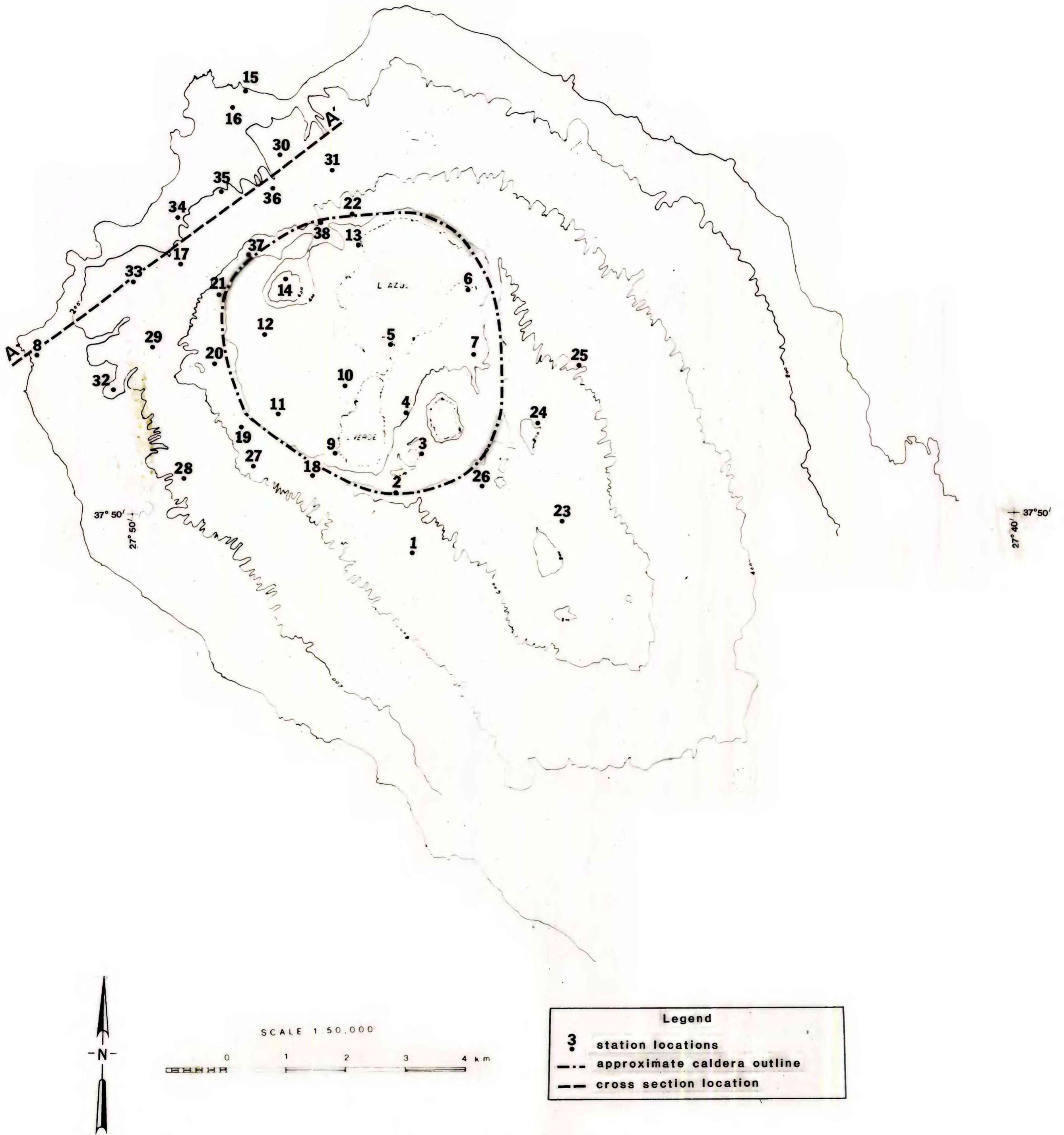
Plate 1. Audio-magnetotelluric station location map for Sete Cidades area São Miguel Island, Azores
