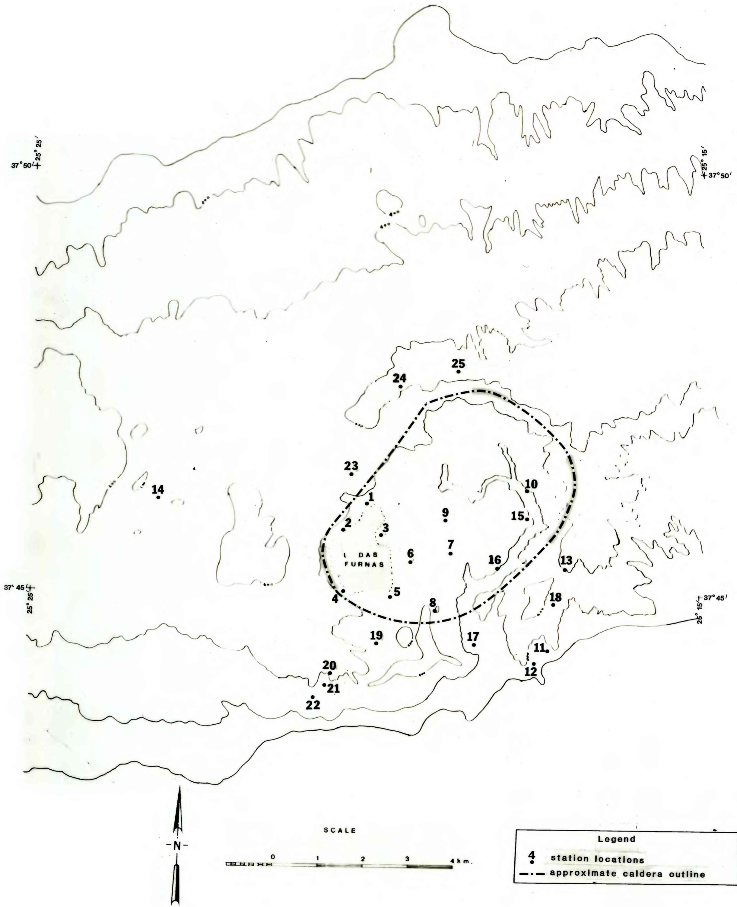
Plate 2. Audio-magnetotelluric station location map for Furnas area, São Miguel Island, Azores
