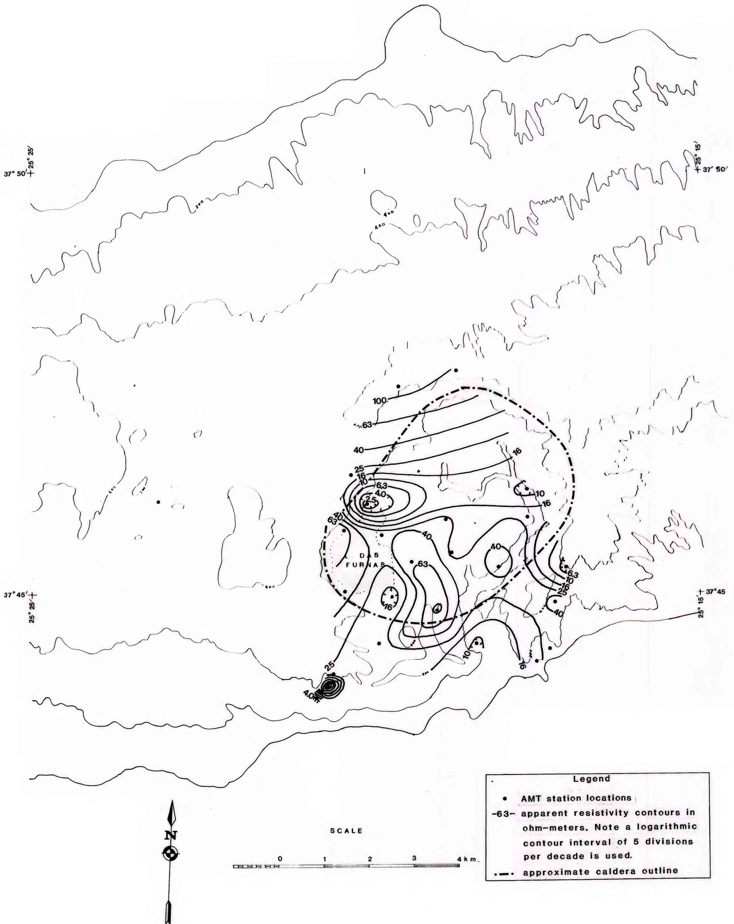
Plate 3. Audio-magnetotelluric scalar apparent resistivity map at 7.5 Hz for a NW-SE orientation of the telluric dipole for the Furnas area, São Miguel Island, Azores
