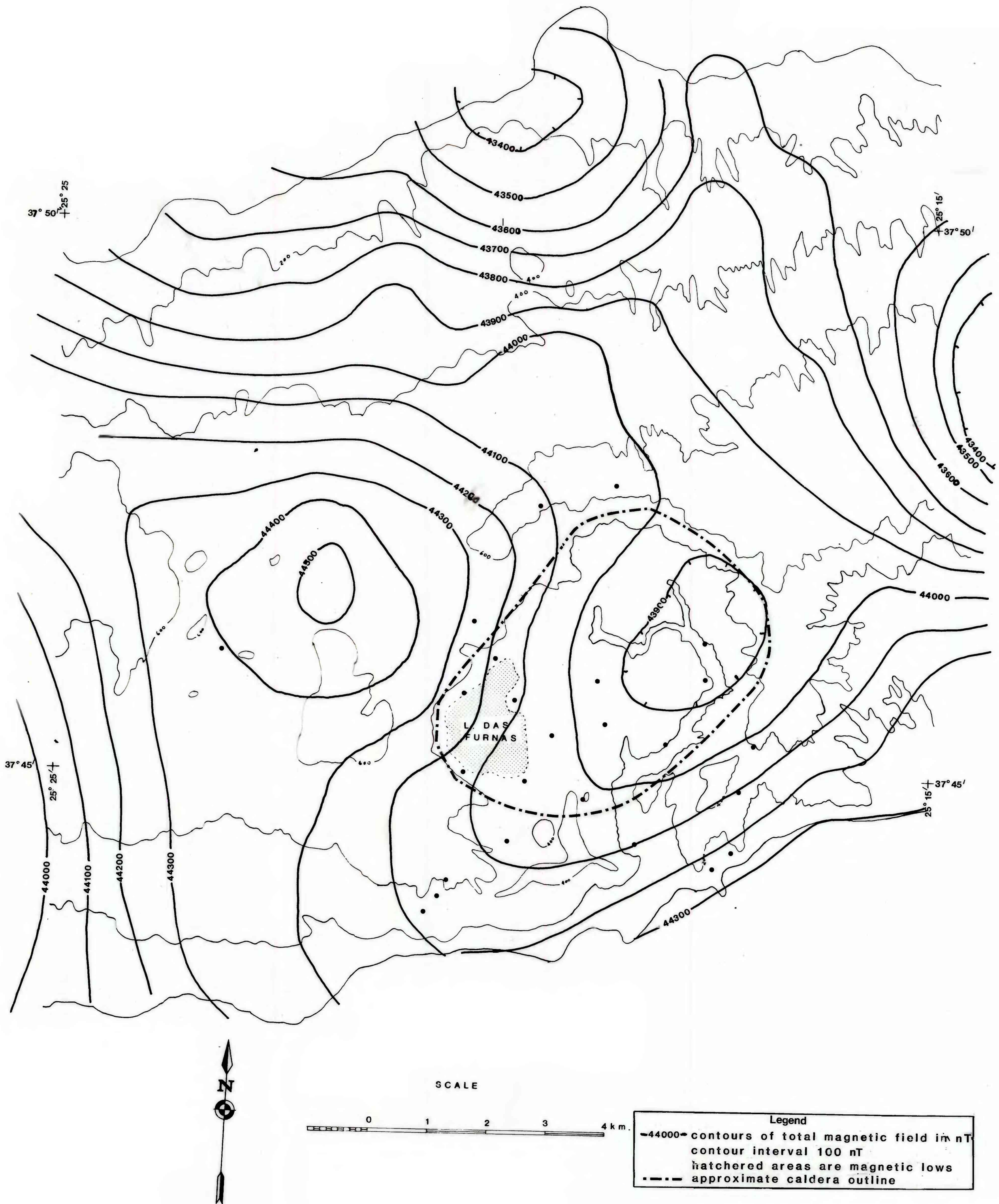
Plate 5. Total field aeromagnetic map of the Furnas area, São Miguel Island, Azores
