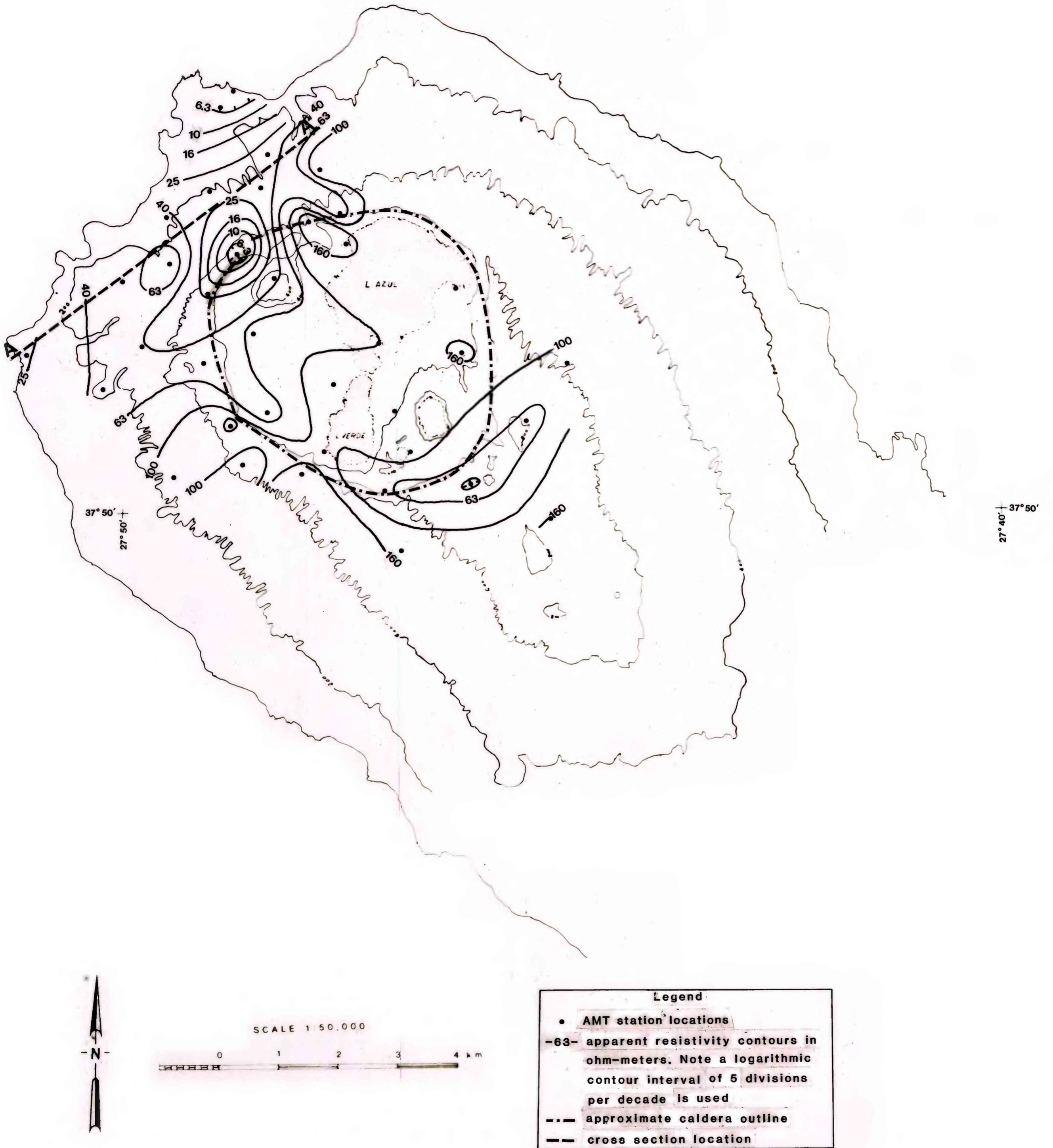
Plate 7. Audio-magnetotelluric scalar apparent resistivity map at 7.5 Hz for a NE-SW orientation of the telluric dipole for the Sete Cidades area São Miguel Island, Azores
