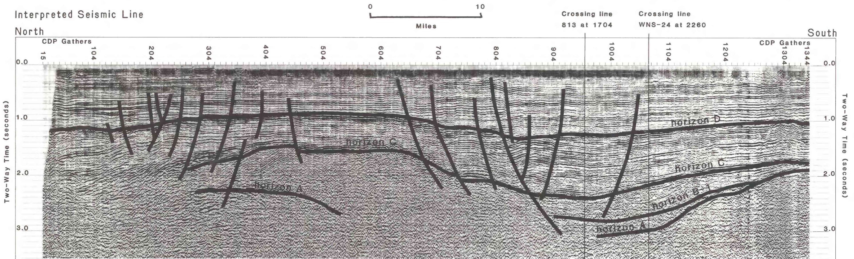
Figure 8. USGS Seismic Line 807.
