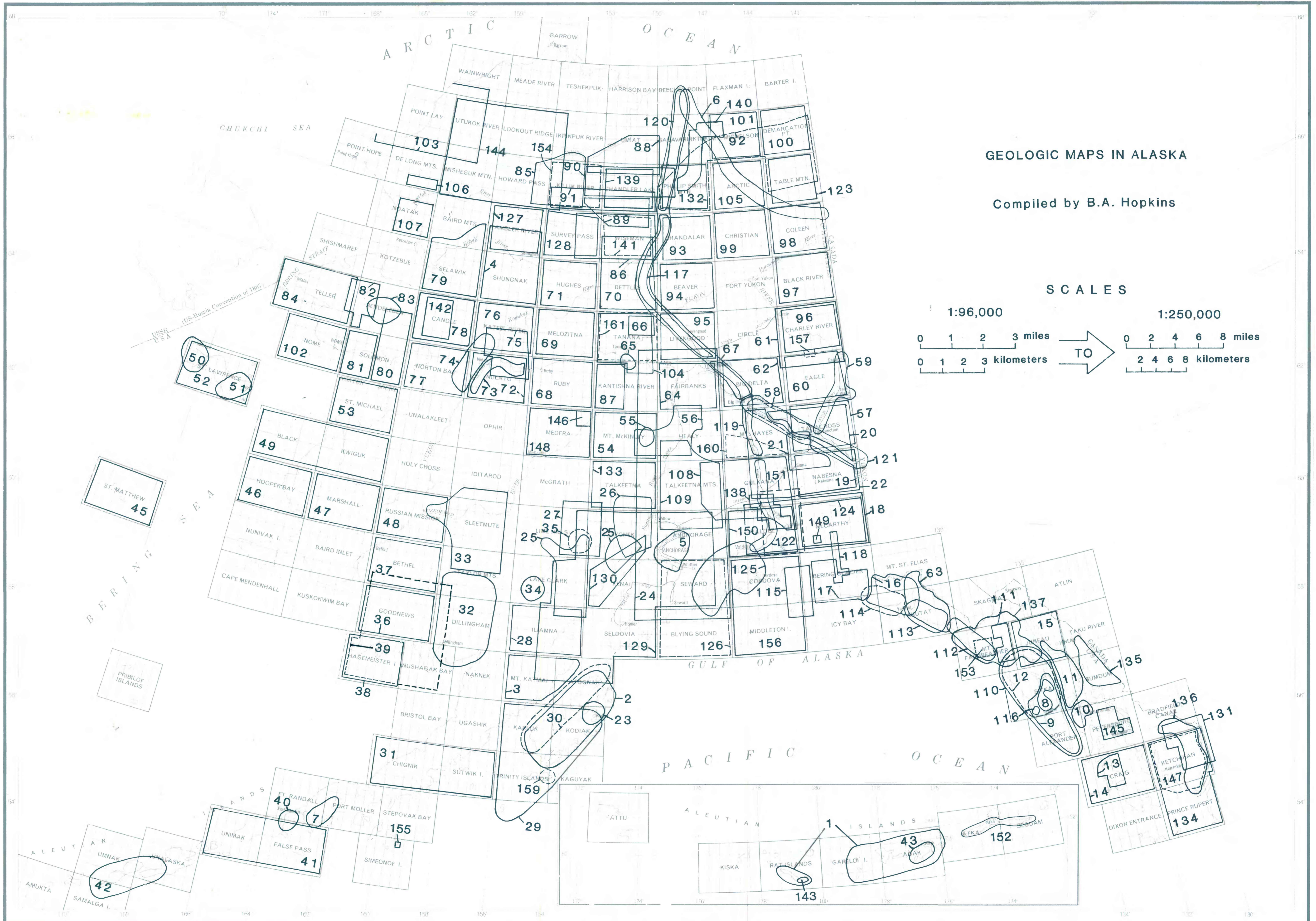
GEOLOGIC MAPS IN ALASKA Scales 1:96,000 to 1:250,000 Compiled by B.A. Hopkins
