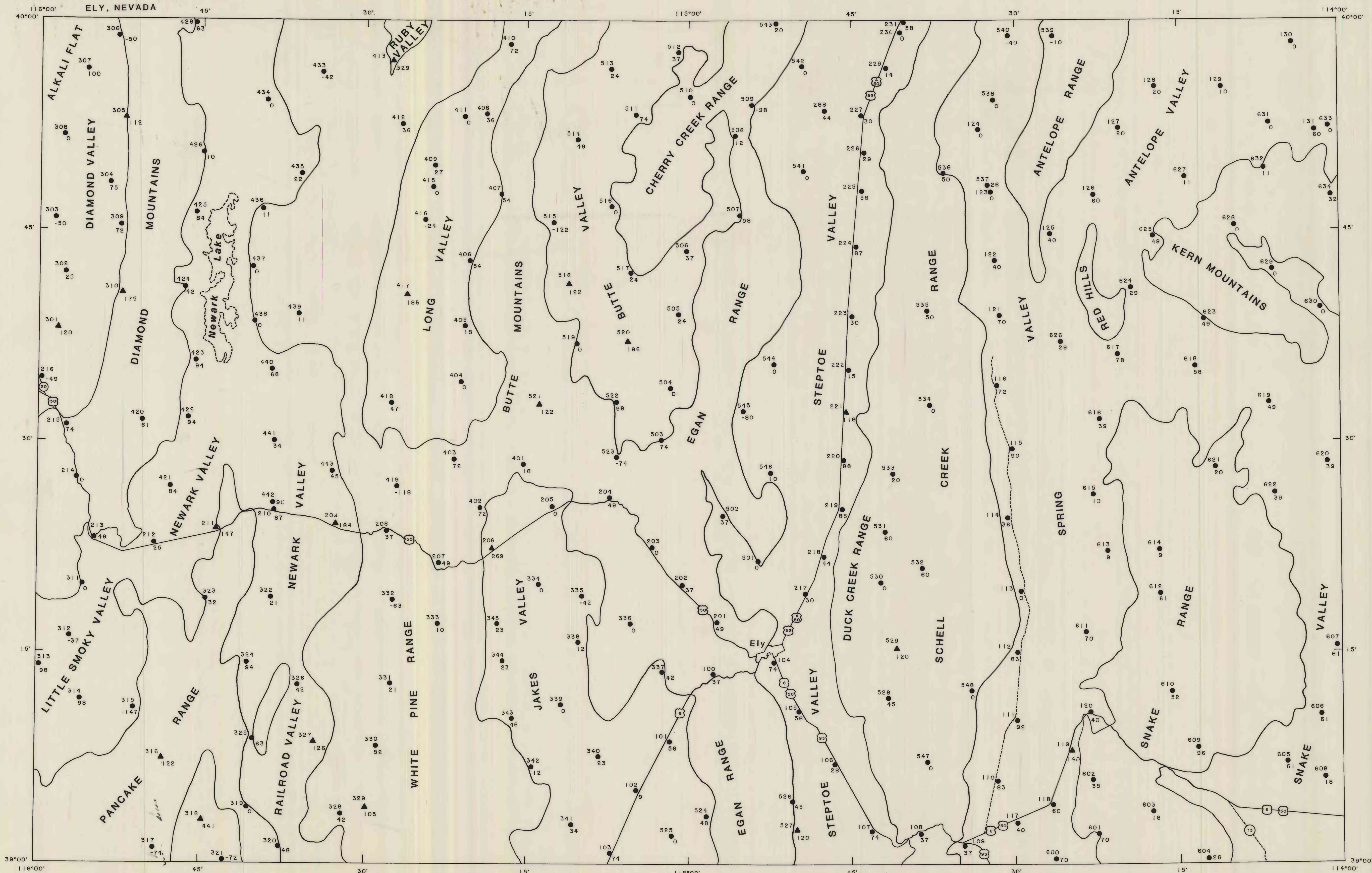
Plate 1.--Map showing principal topographic features and helium concentrations in soil-gas samples, Ely, Nevada 1° x 2° quadrangle.
