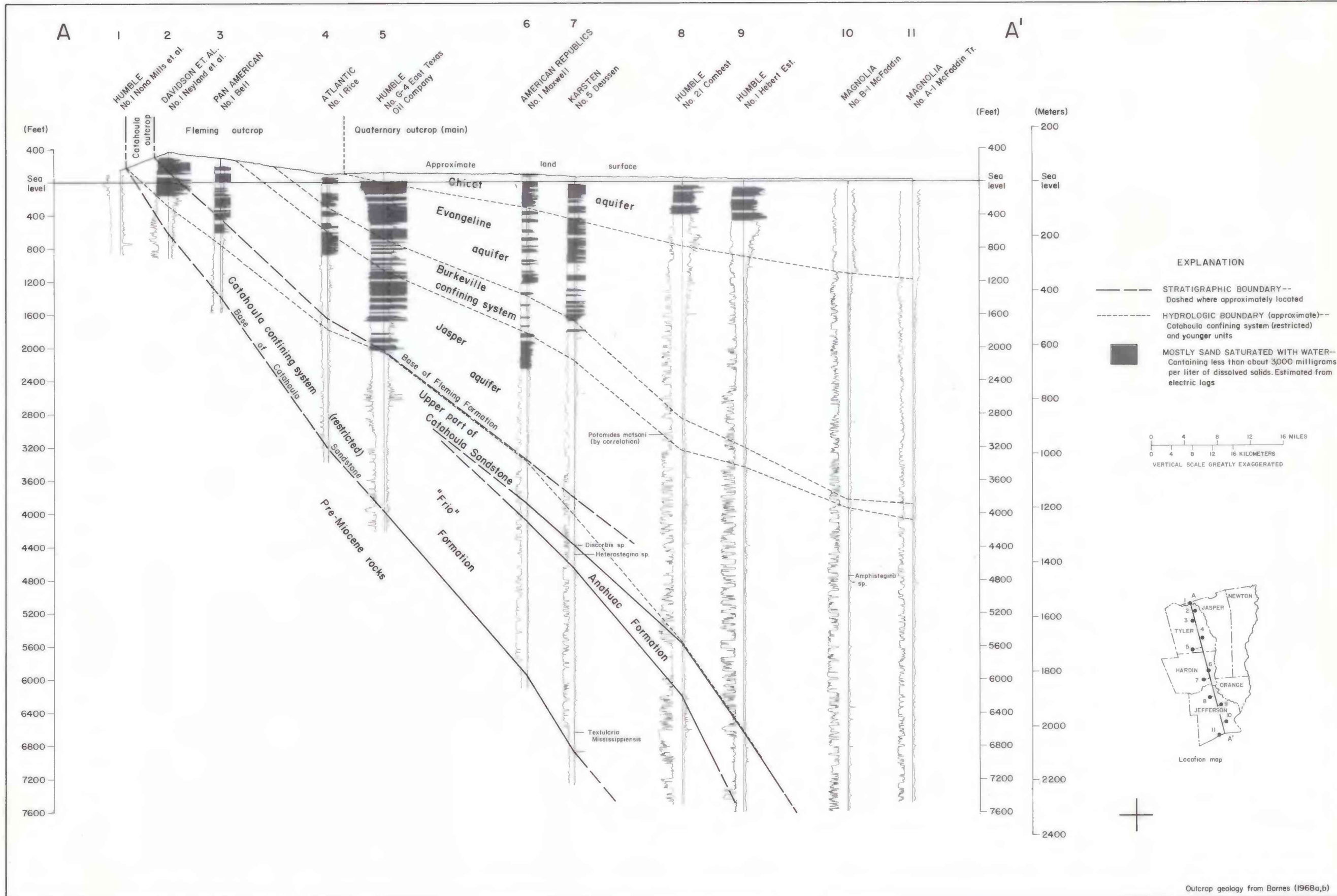
Figure 3.-Stratigraphic and hydrologic section, A-A'.
