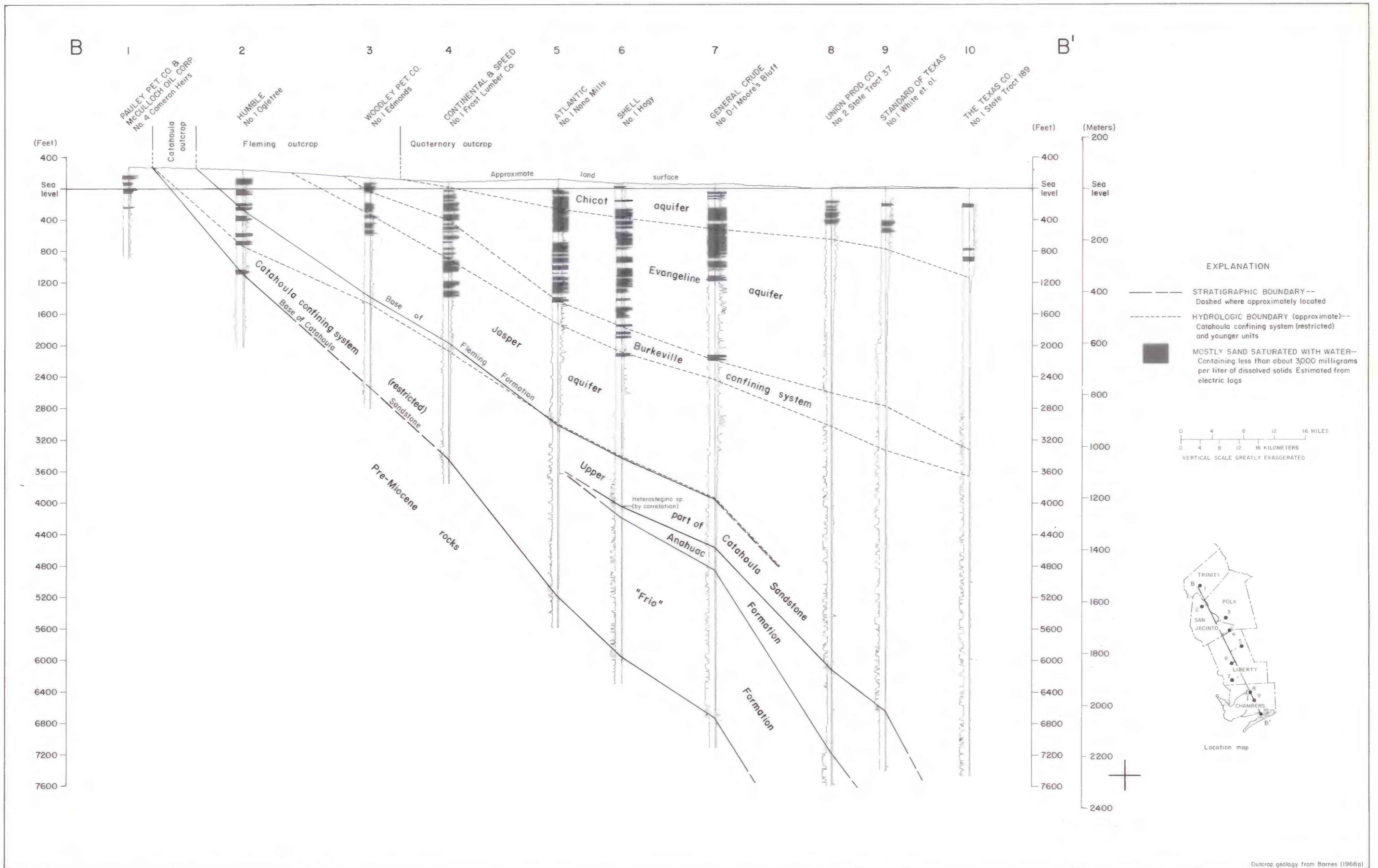
Figure 4.—Stratigraphic and hydrologic section, B-B'
