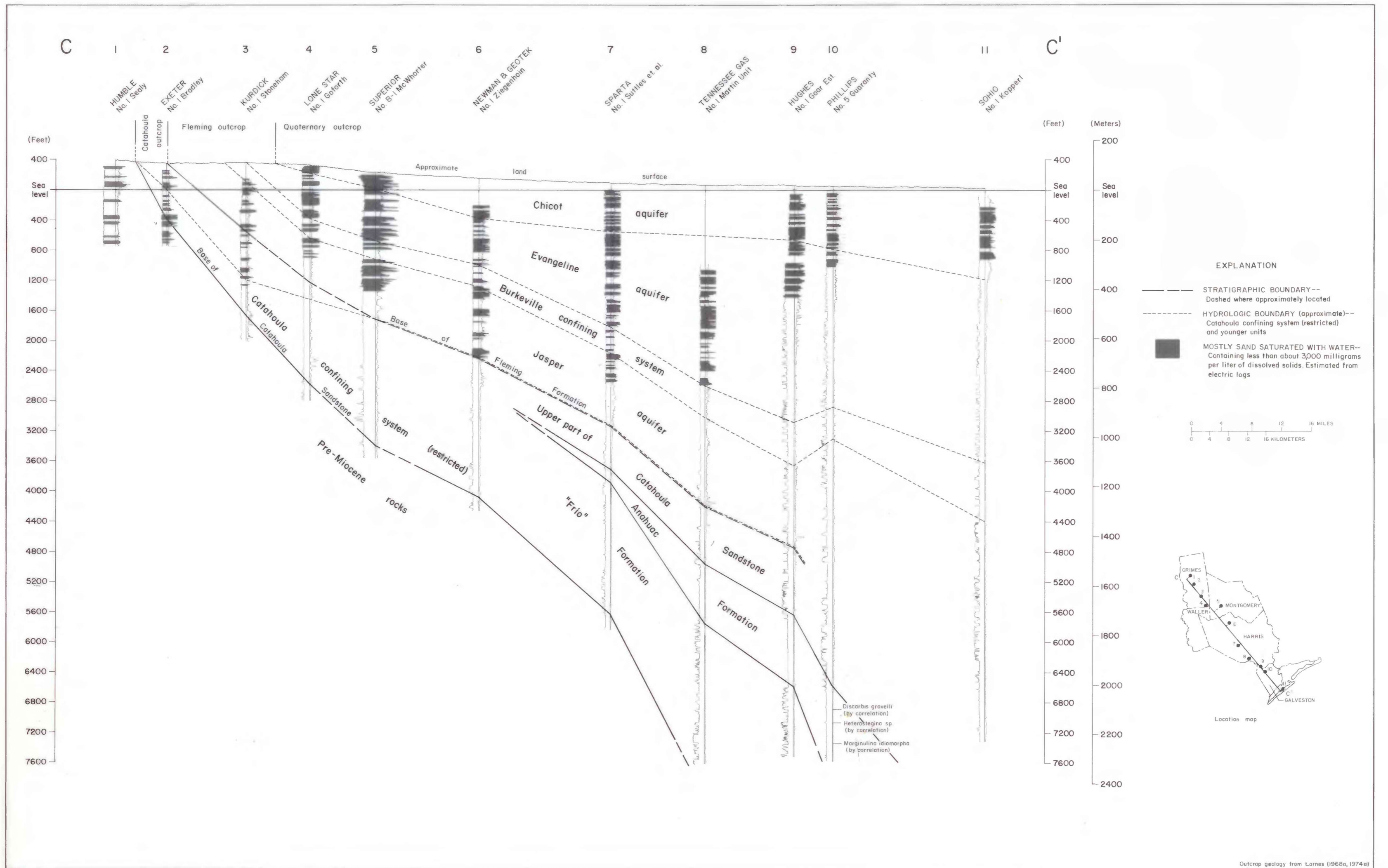
Figure 5.—Stratigraphic and hydrologic section, C-C'.
