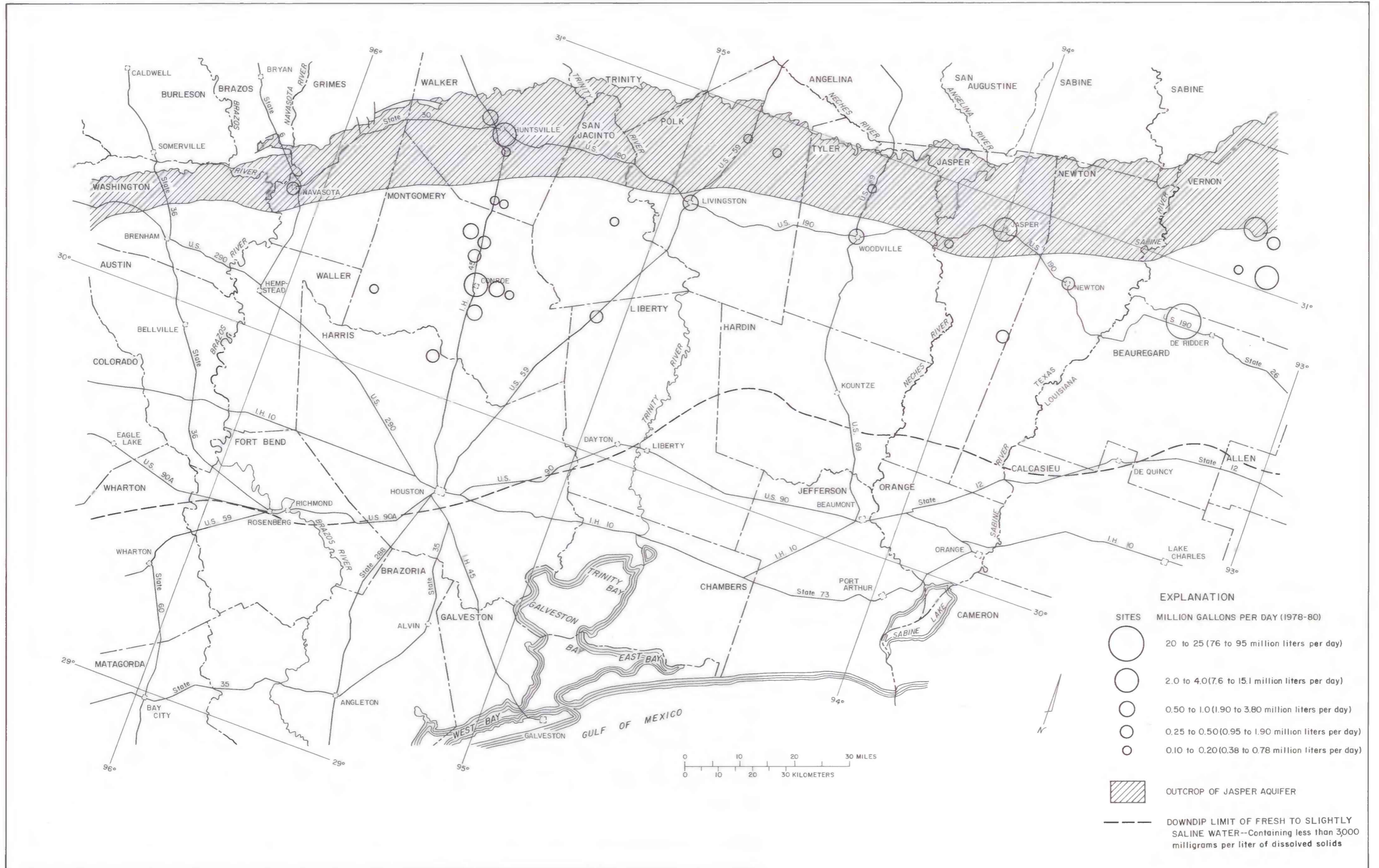
Figure 9.—Sites where moderate to large volumes of water are pumped from the Jasper aquifer.
