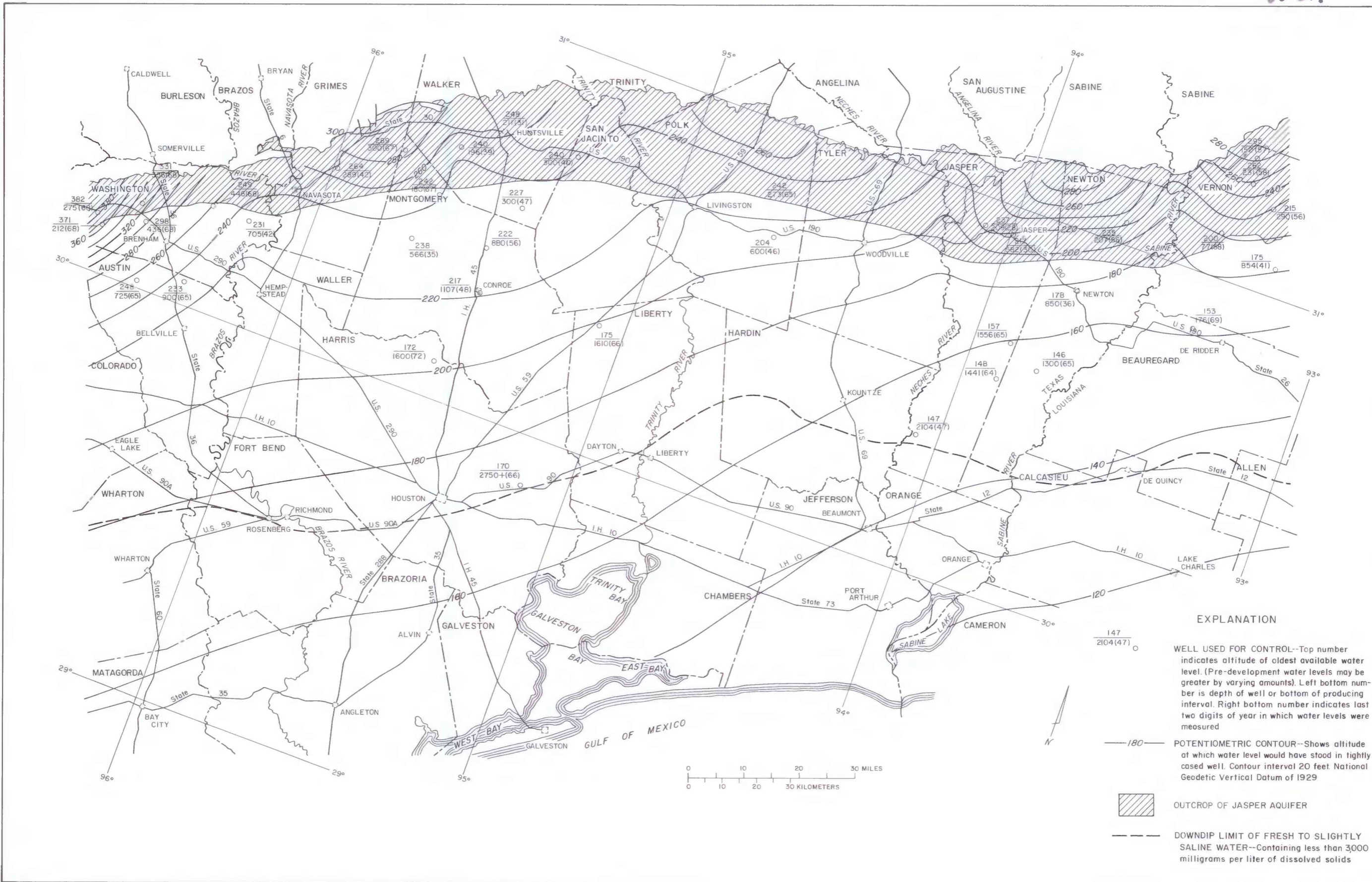
Figure 11.—Approximate potentiometric surface of the Jasper aquifer prior to development by wells.
