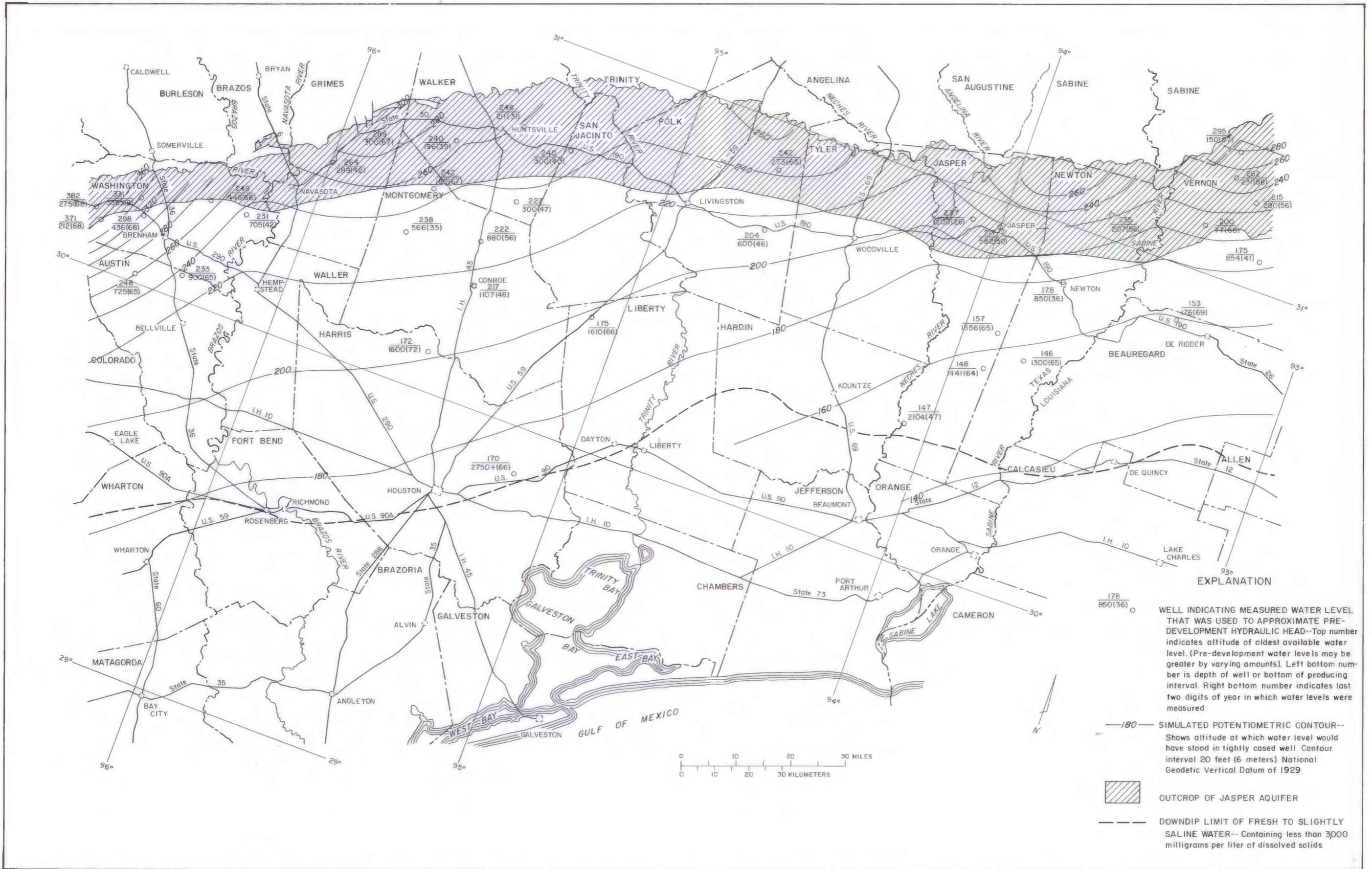
Figure 19.--Simulated potentiometric surface of the Jasper aquifer prior to development by wells.
