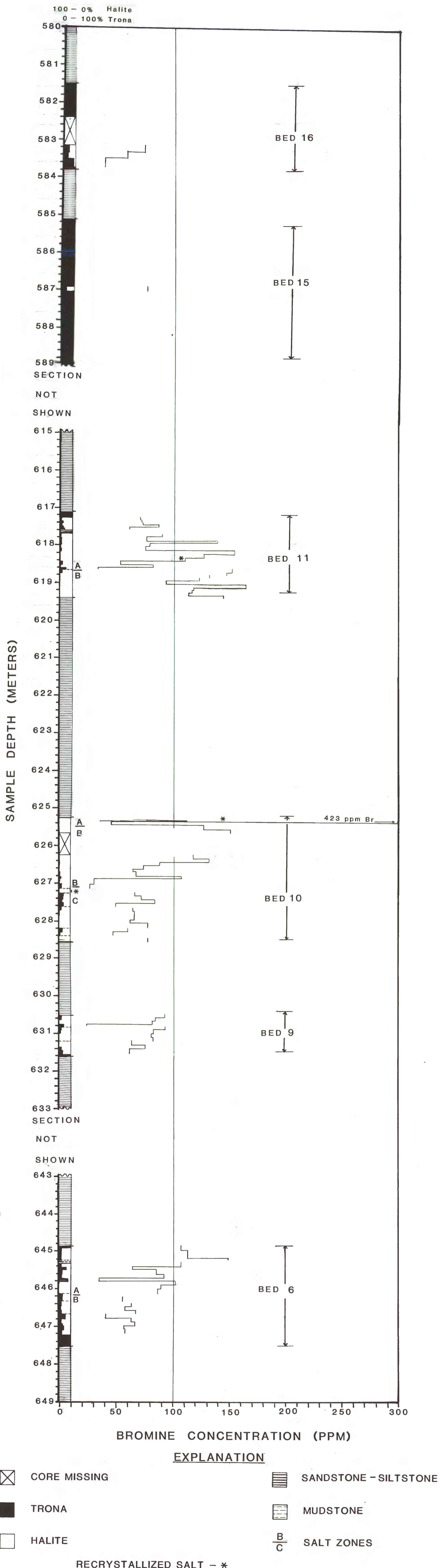
Plate 1.--BROMINE PROFILES OF HALITE BEDS 6, 9, 10, 11, 15, AND 16 IN FINLEY 2 DRILL HOLE by Debra K. Higley 1983
