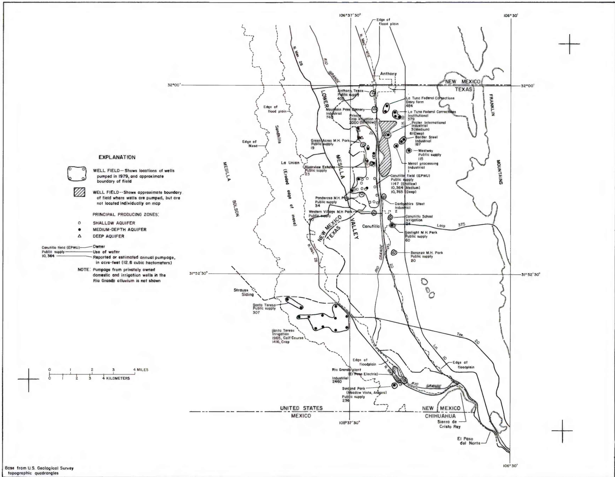
Figure 3.—Well-field area and ground-water withdrawals, lower Mesilla Valley, 1979
