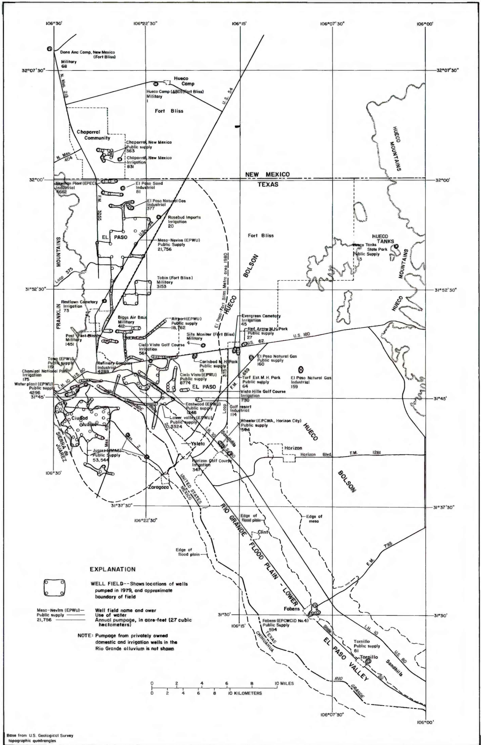
Figure 4.-Well-field areas and ground-water withdrawals, Hueco bolson, 1979
