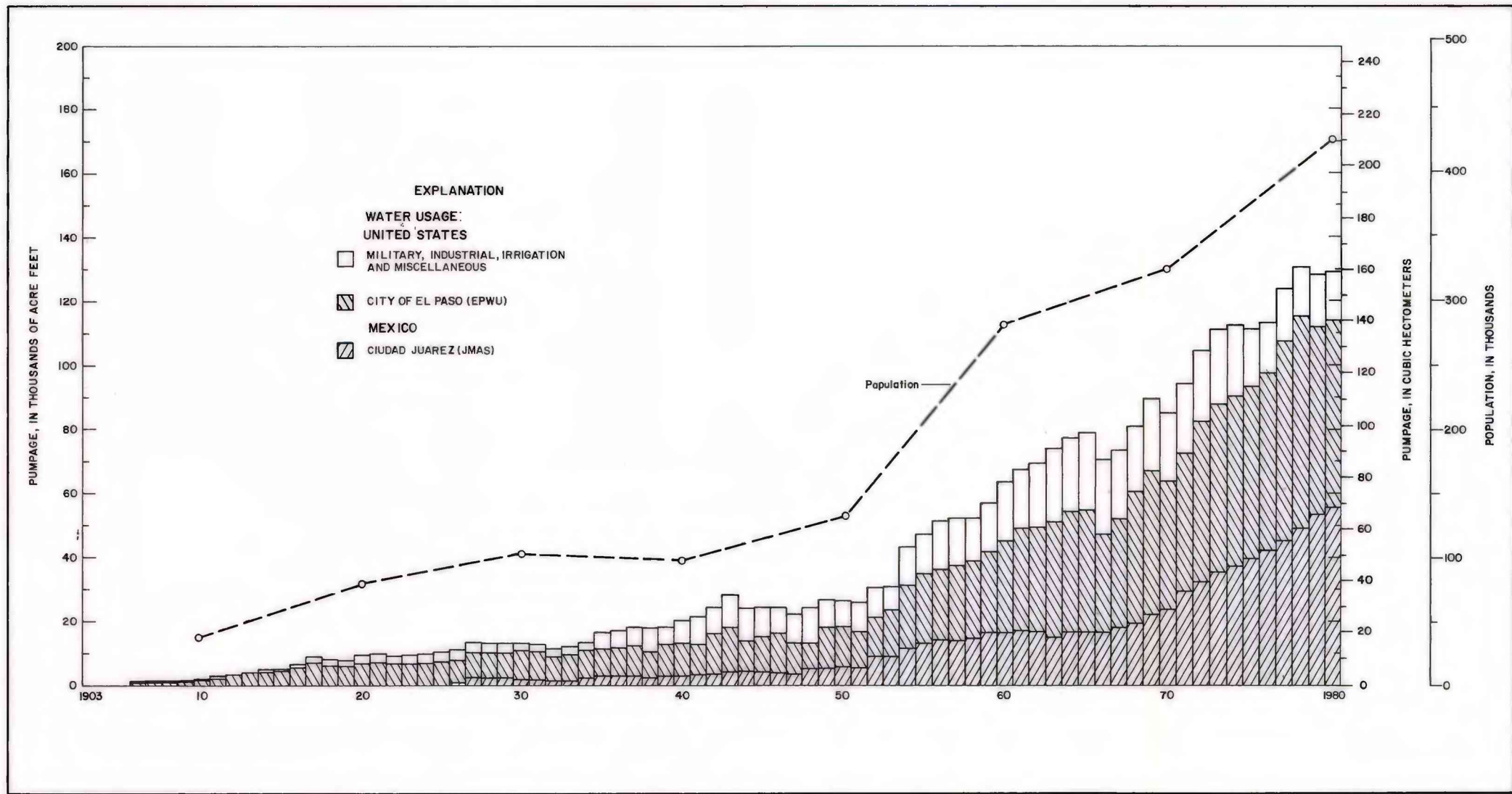
Figure 13.-Withdrawals of ground water from the Hueco bolson metro area, 1906-80 and 10-year census population for the city of El Paso
