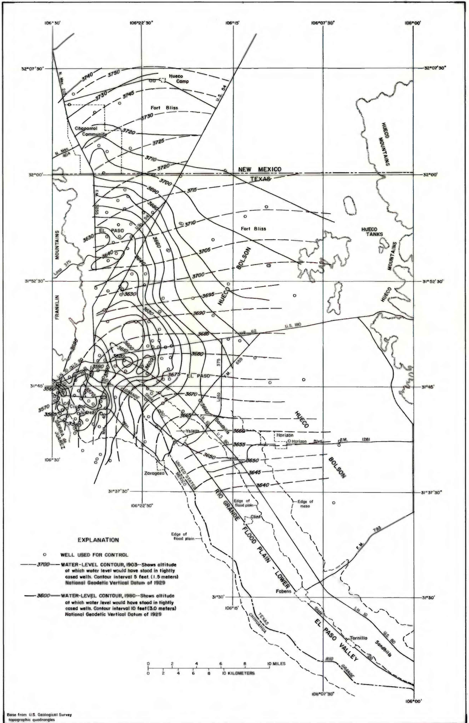
Figure 14.—Approximate altitude of water levels in the Hueco bolson, 1903 and January 1980
