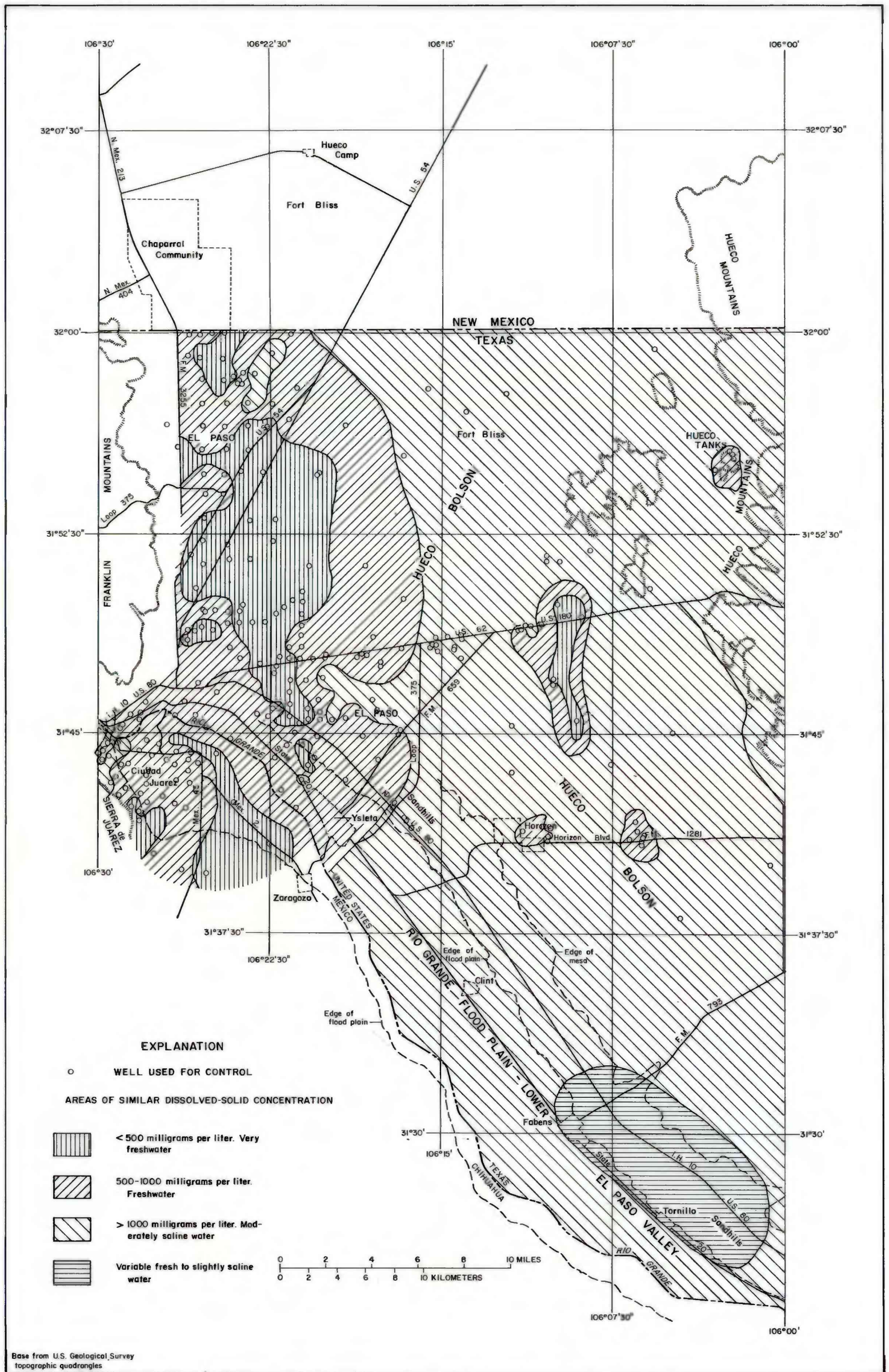
Figure 18.—Areas of similar dissolved-solids concentrations in samples from wells in the Hueco bolson, 1979-81
