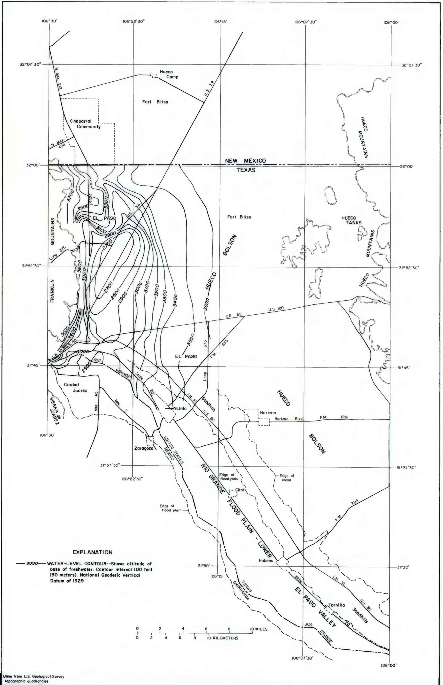
Figure 35.—Approximate altitude of the base of freshwater in the Hueco bolson, 1973
