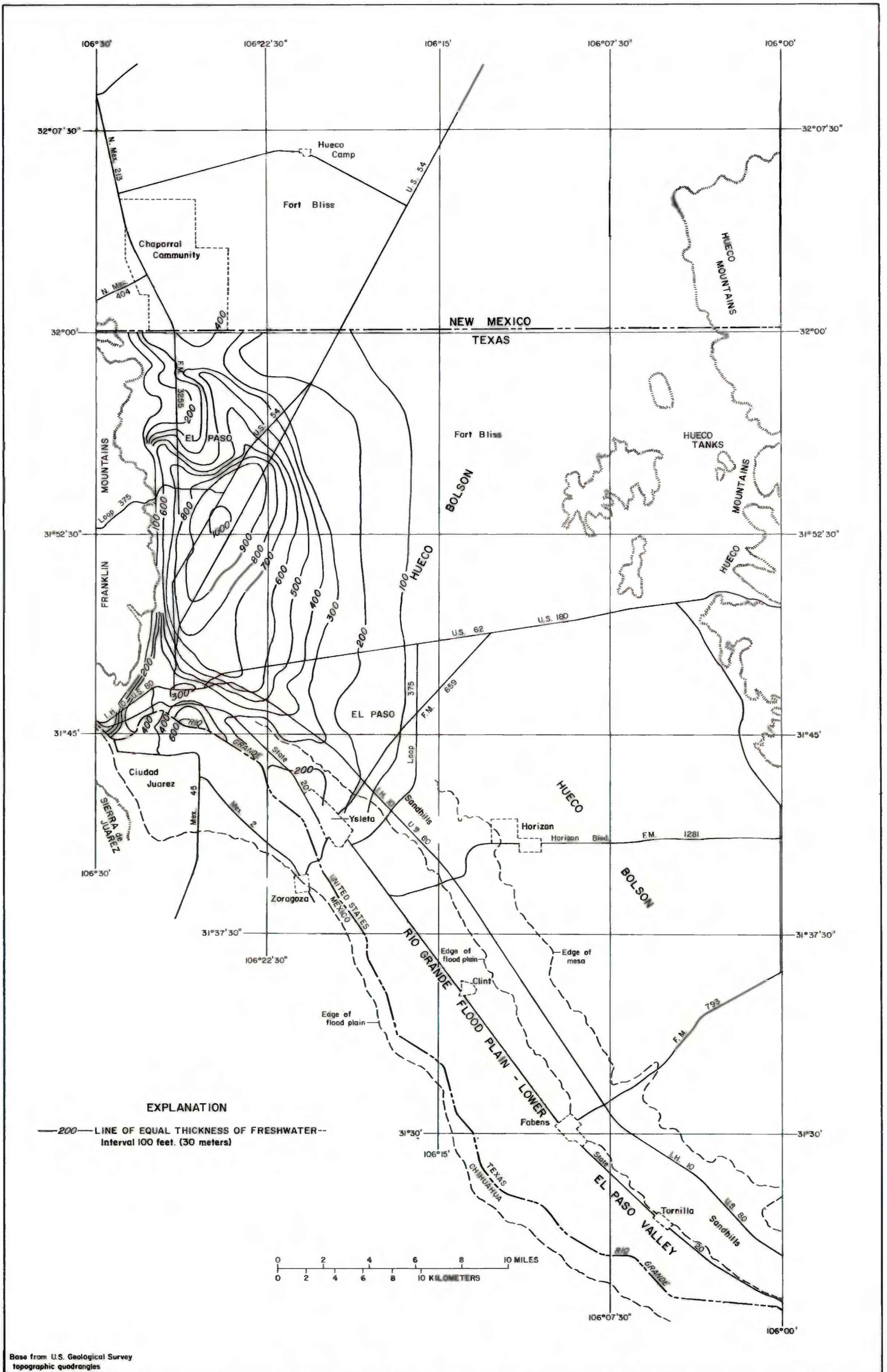
Figure 36 - Estimated thickness of sediments containing freshwater in the Hueco bolson, January 1980
