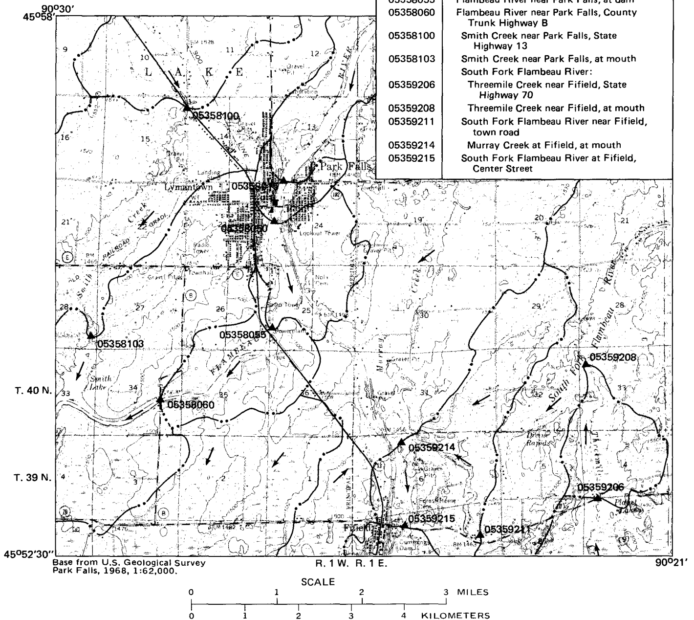
Figure 1. Typical stream network and tabular listing.
