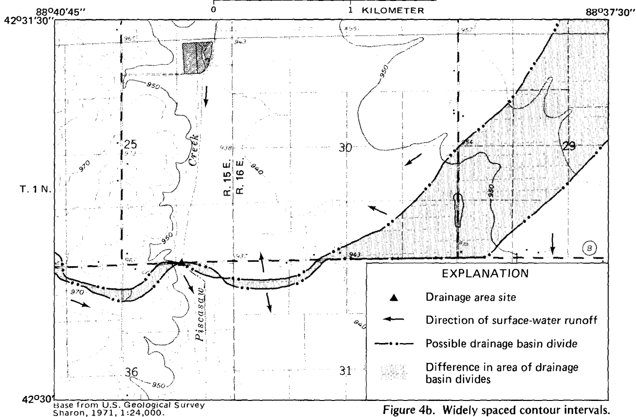
Figure 4. Example of topographic divide determination.
