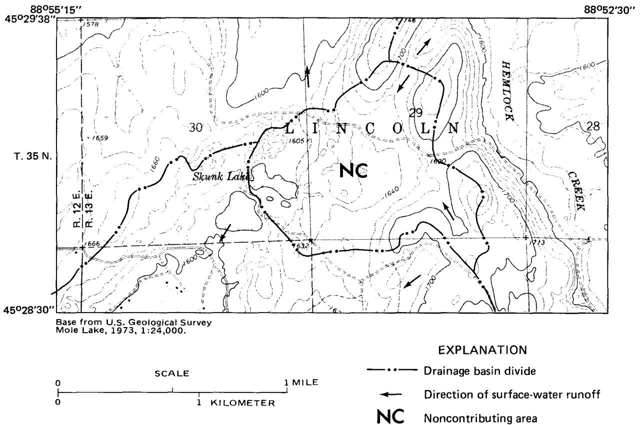
Figure 3. Example of topographic map showing an area that does not contribute surface-water runoff directly to a stream.
