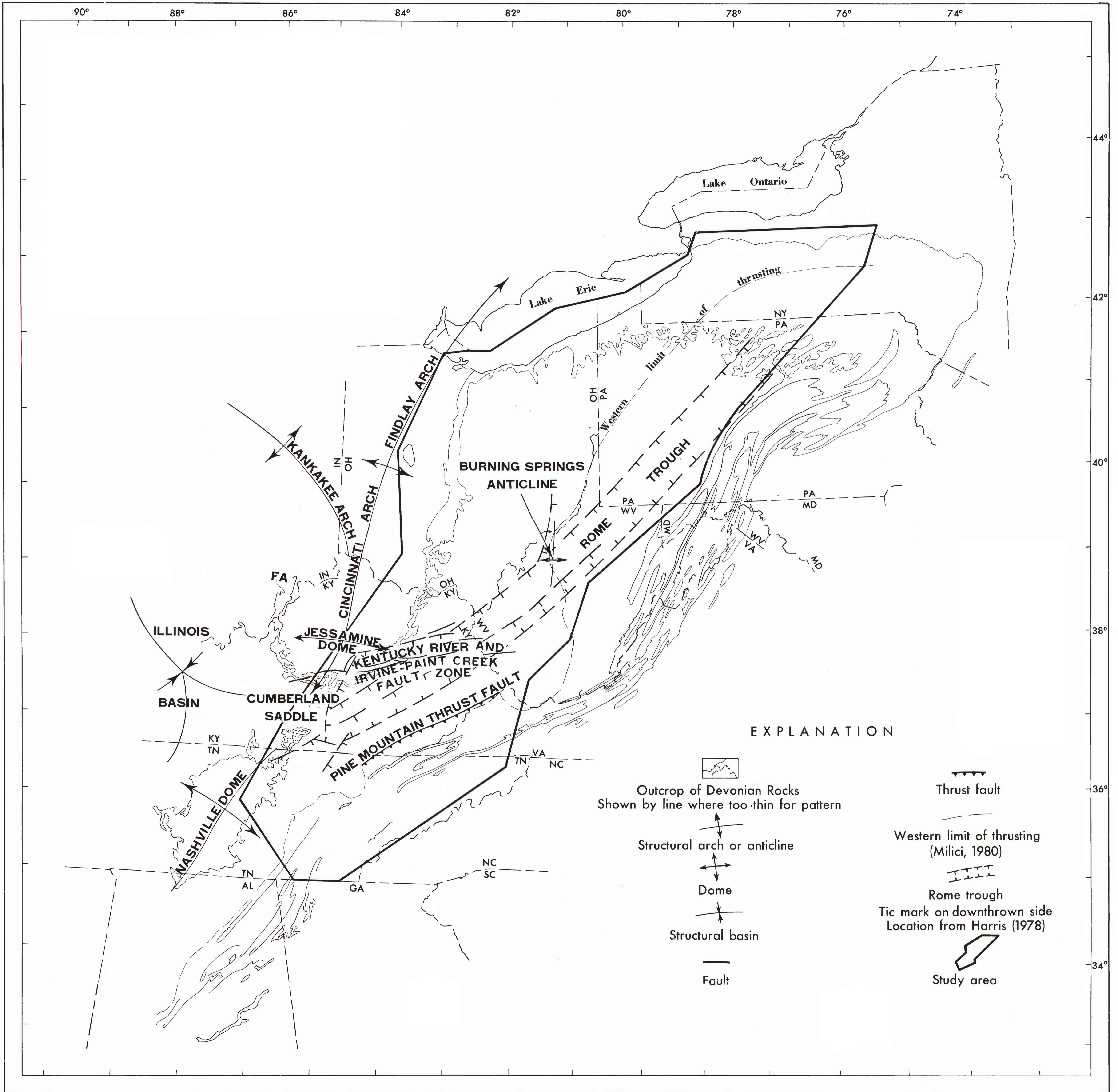
INDEX MAP SHOWING AREA OF STUDY, OUTCROP OF ROCKS OF DEVONIAN AGE AND MAJOR STRUCTURAL FEATURES OF THE APPALACHIAN BASIN
