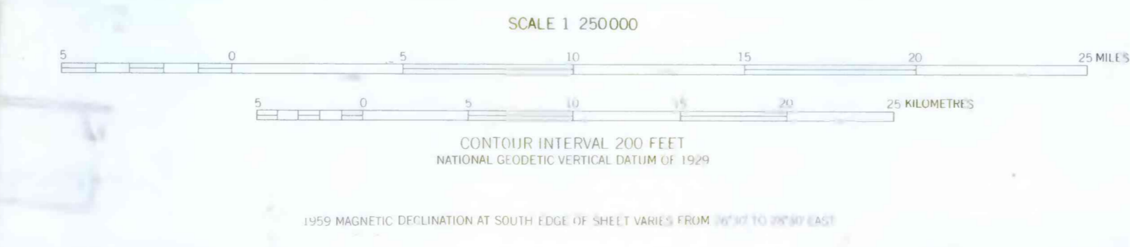
This map is preliminary and has not been edited or reviewed for conformity with Geological Survey editorial standards or stratigraphic nomenclature. MAP SHOWING SITES AT WHICH STREAM-SEDIMENT AND PEBBLE SAMPLES WERE COLLECTED FROM THE WISEMAN QUADRANGLE, ALASKA
