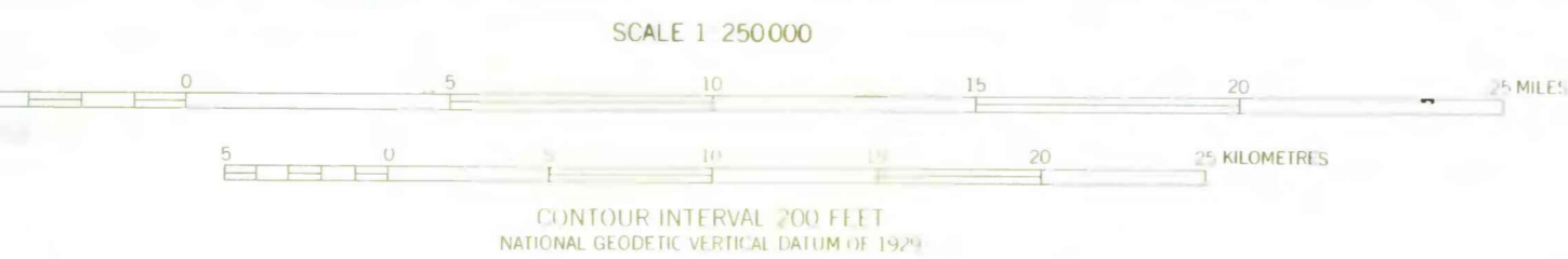
This map is preliminary and has not been edited or reviewed for conformity with Geological Survey editorial standards or stratigraphic nomenclature. MAP SHOWING SITES AT WHICH ROCK SAMPLES WERE COLLECTED FROM THE WISEMAN QUADRANGLE, ALASKA
