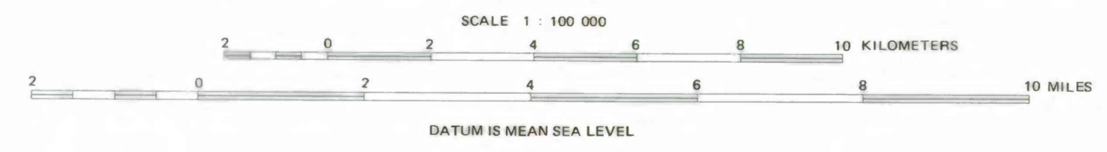
MAP OF THE JANBAN QUADRANGLE, SHEET 20/44 B, KINGDOM OF SAUDI ARABIA, SHOWING SAMPLE LOCATIONS, ROCK TYPES, AND GEOGRAPHIC AND CULTURAL FEATURES by Maurice R. Brock 1984
