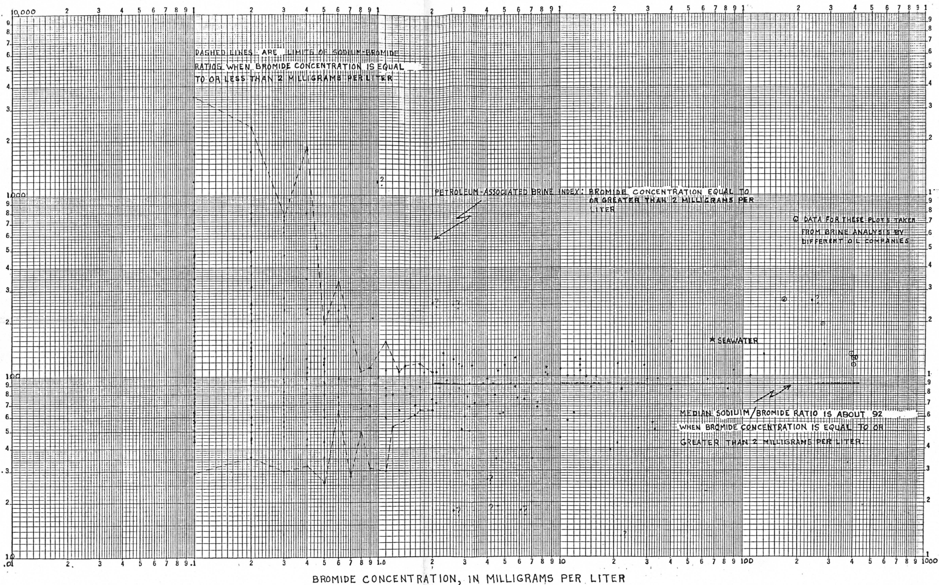
Figure 2. - Relation of sodium bromide ratios to bromide concentrations. Questioned points may or may not be valid, see text.
