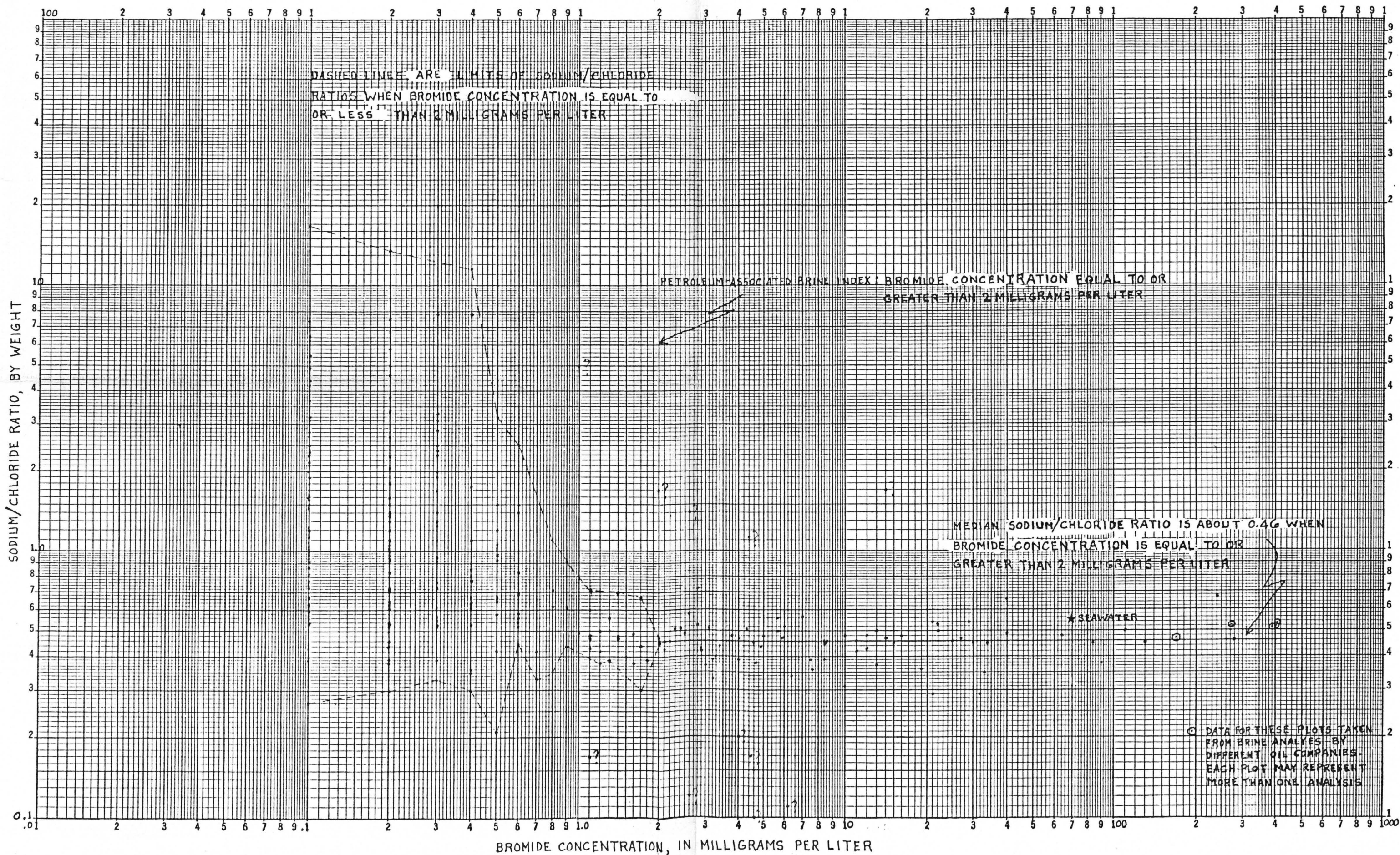
Figure 3. - Relation of sodium/chloride ratios to bromide concentrations. Questioned points may or may not be valid, see text.
