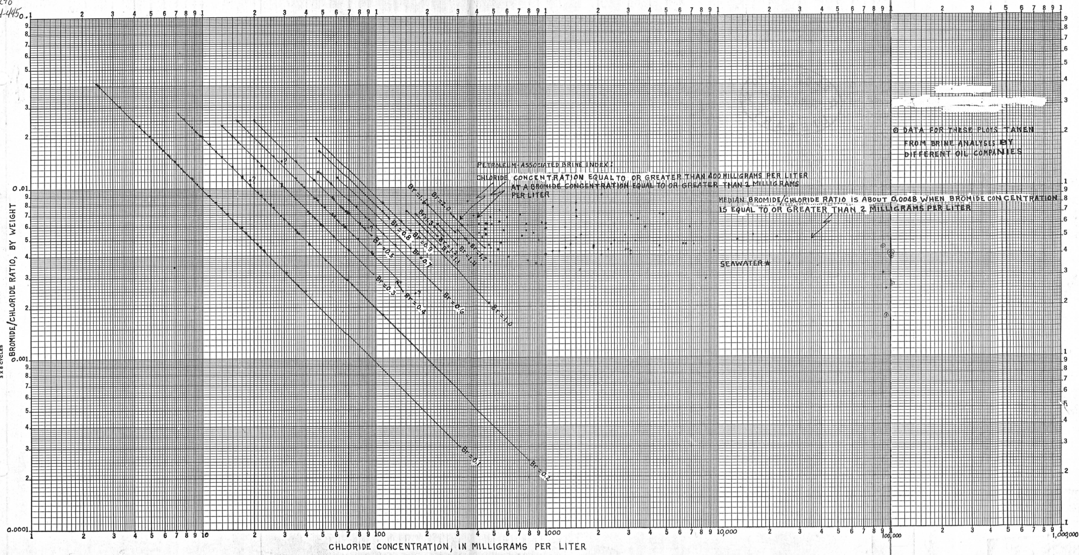
Figure 4.- Relation of bromide/chloride ratios to chloride concentrations. questioned points may or may not be valid - see text.
