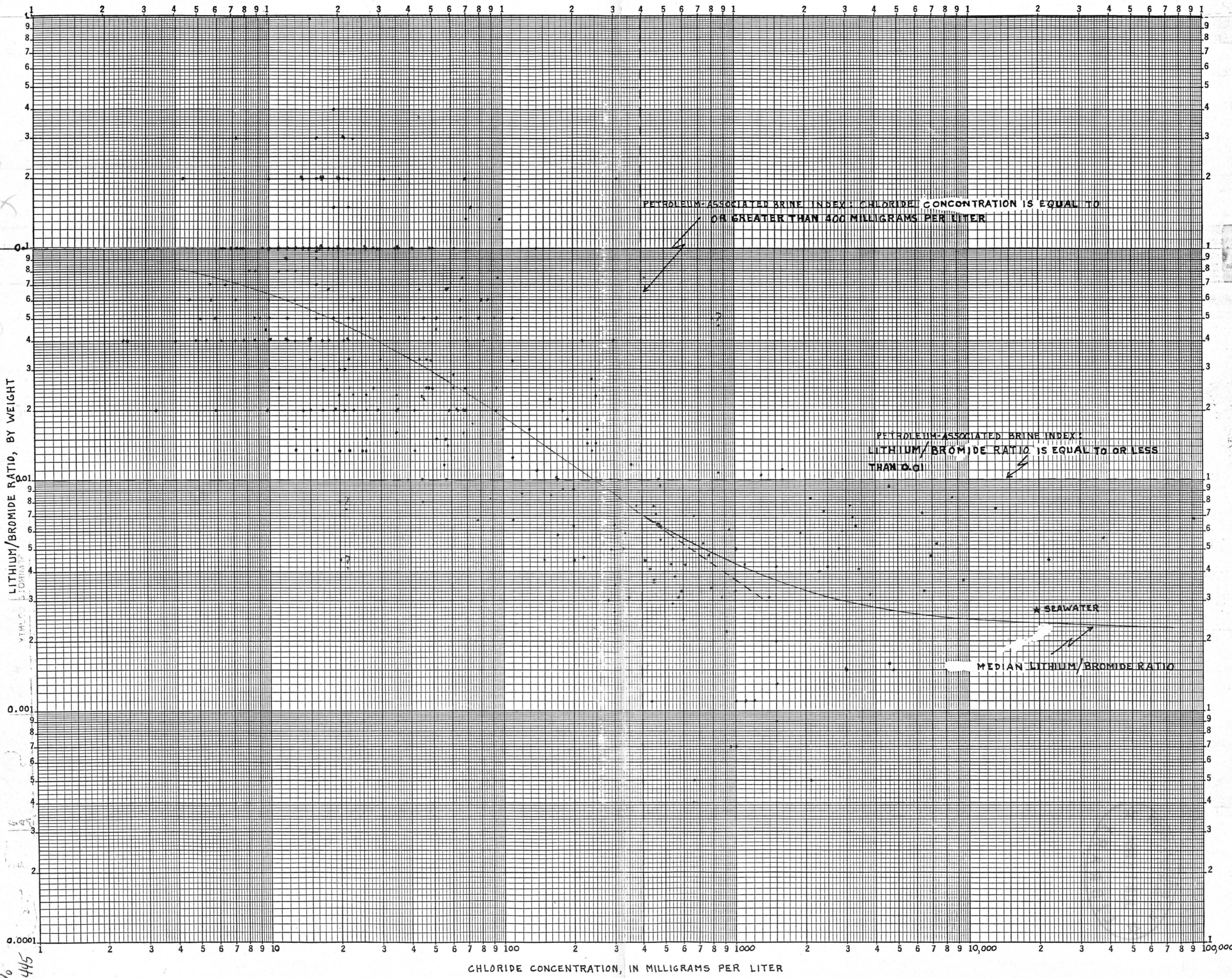
Figure 7. - Relation of lithium/bromide ratios to chloride concentrations. Questioned points may or may not be valid; see text.
