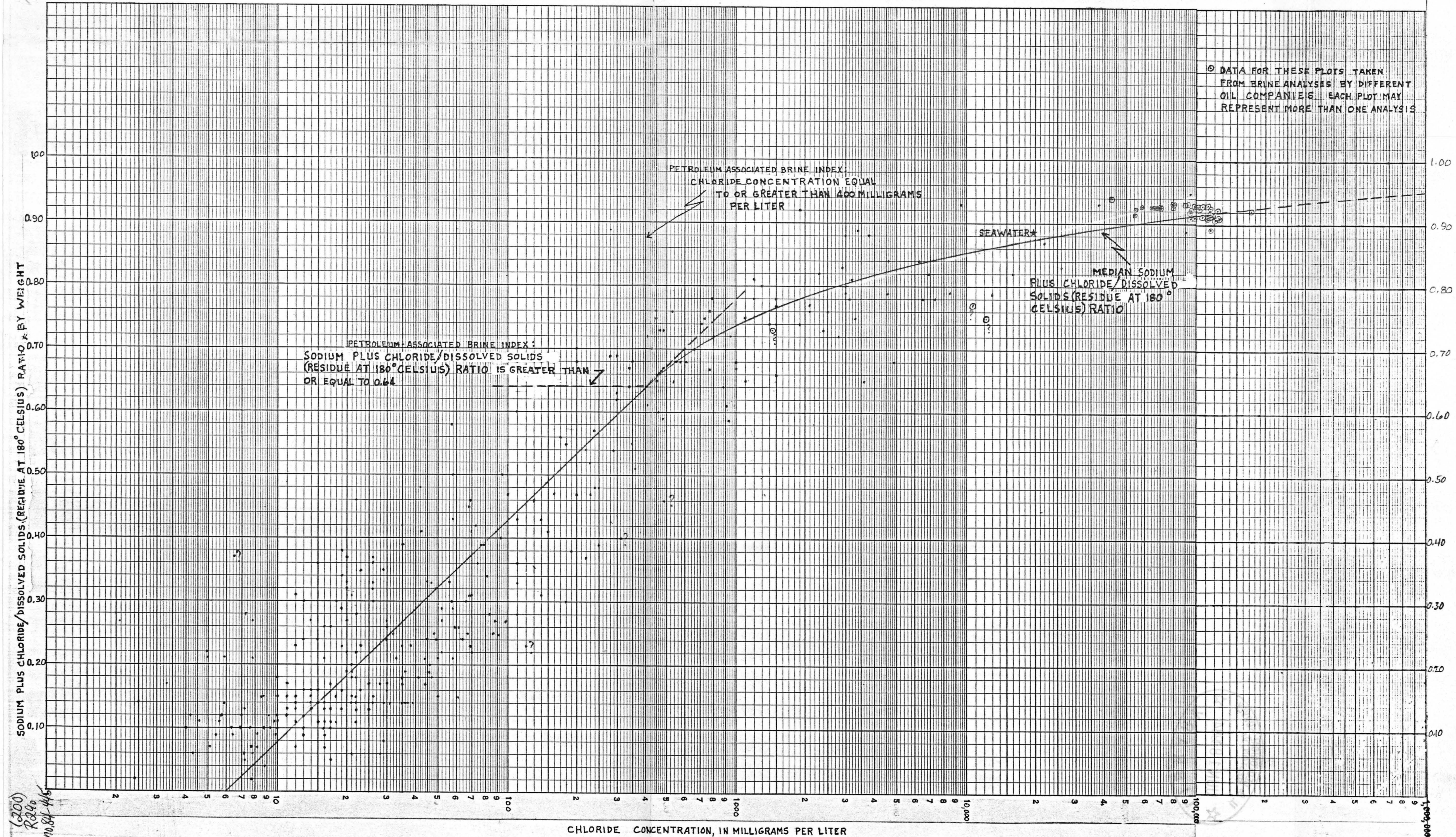
Figure 9.- Relation of sodium plus chloride/dissolved solids (residue at 180° Celsius) ratios to chloride concentrations. Questioned points may or may not be valid, see text.
