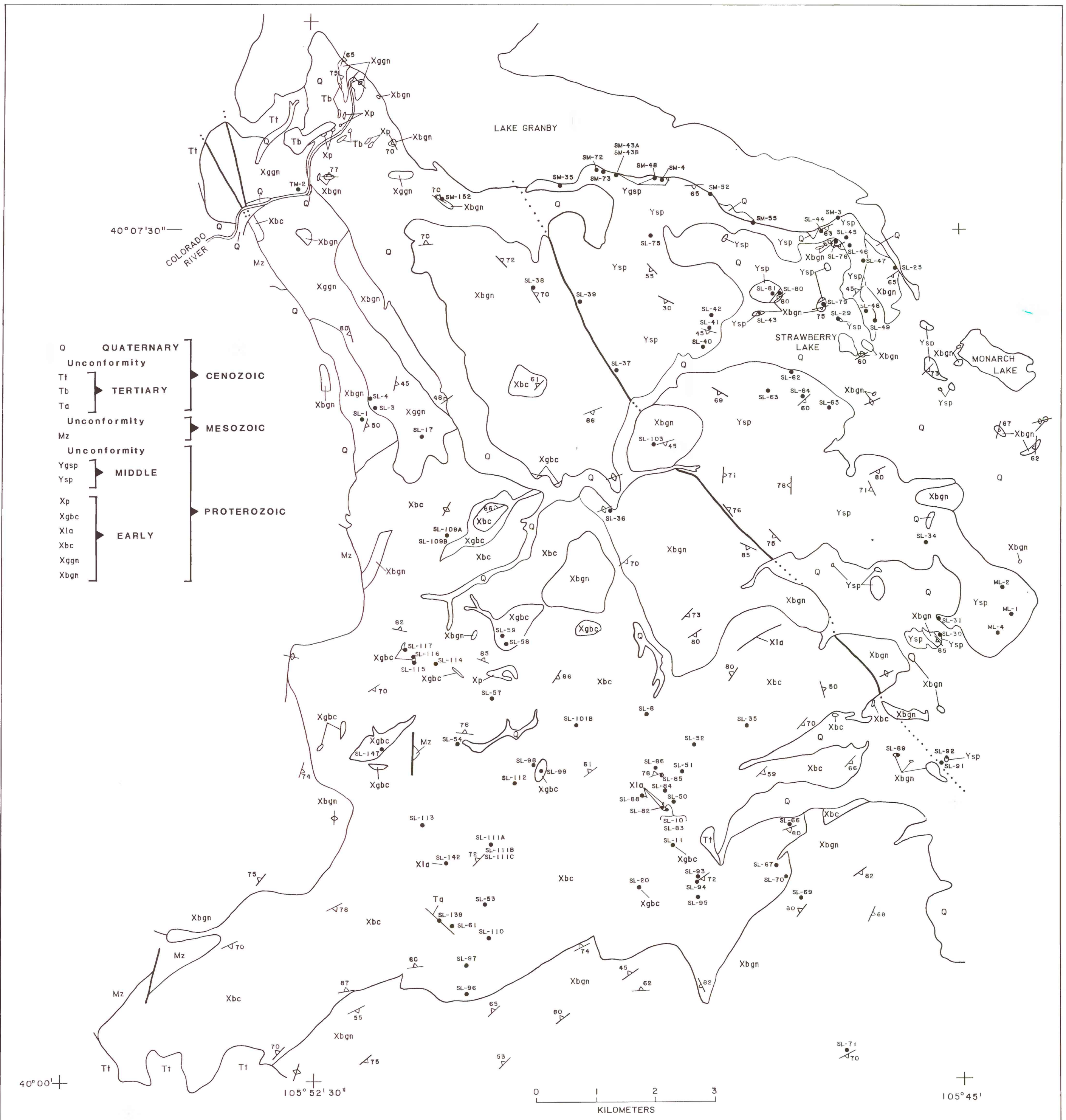
PLATE 1 --GEOLOGIC SKETCH MAP OF THE STRAWBERRY LAKE AREA AND SAMPLING LOCALITIES
