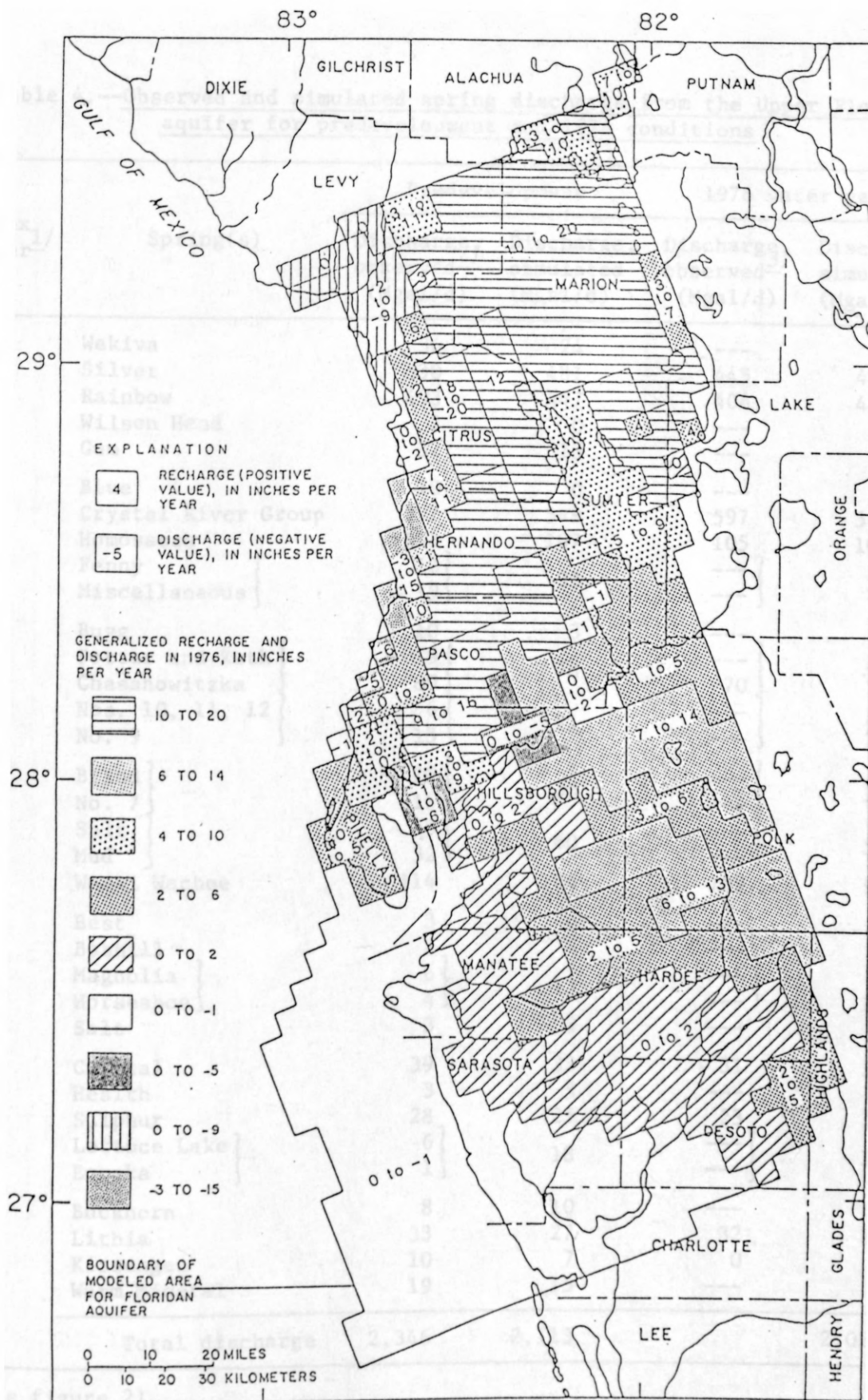
Figure 28a.--Recharge and discharge to the Upper Floridan aquifer in the calibrated model, excluding springflow, 1976.
