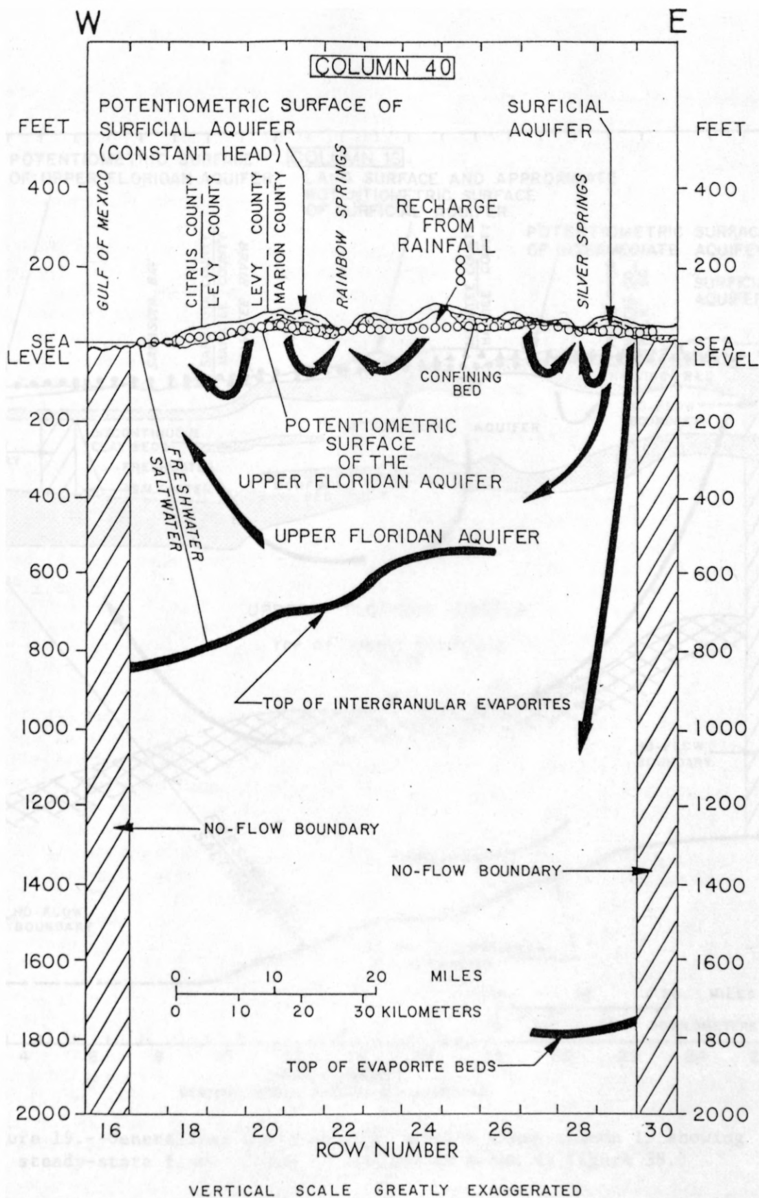
Figure 18.--Generalized hydrogeologic section along column 40 showing steady-state flow. (Line of section is shown in figure 38.)
