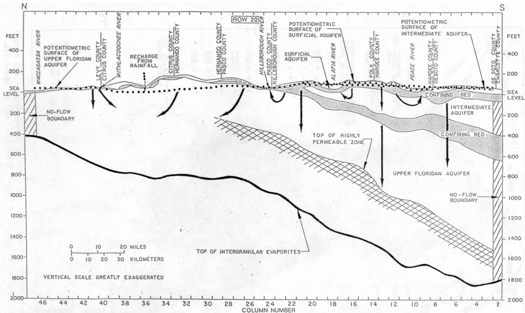
Figure 20.--Generalized hydrogeologic section along row 20 showing steady-state flow nearly perpendicular to flow lines. (Line of section is shown in figure 38.)
