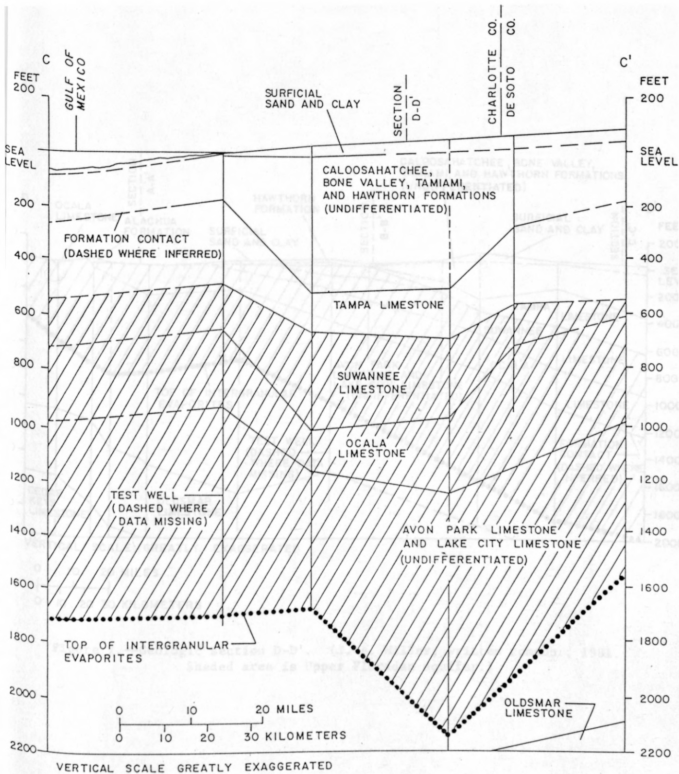
Figure 6.--Geologic section C-C'. (J. A. Miller, written commun., 1981. Shaded area is Upper Floridan aquifer.)
