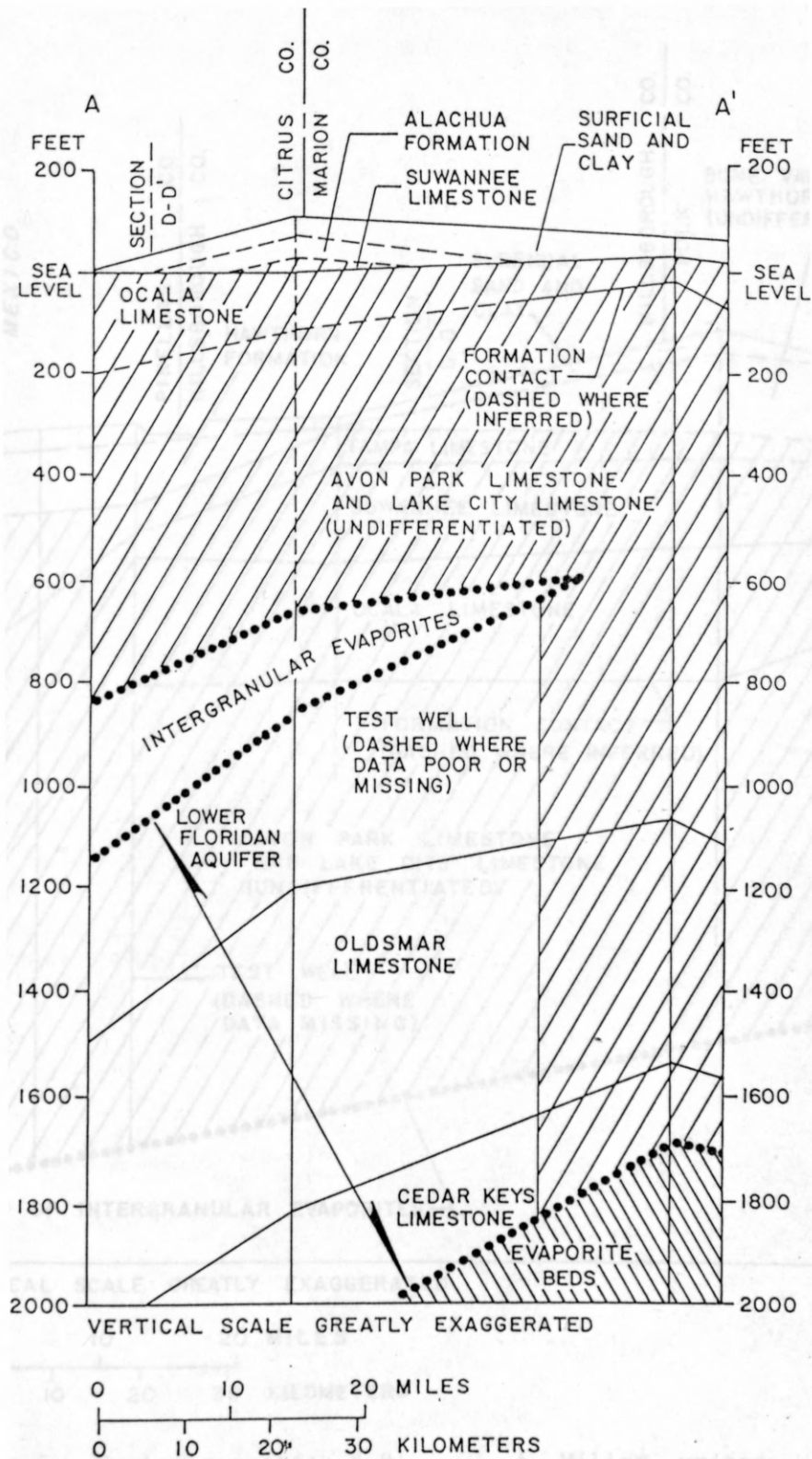
Figure 4.--Geologic section A-A'. (J. A. Miller, written commun., 1981. Shaded area is Upper Floridan aquifer.)
