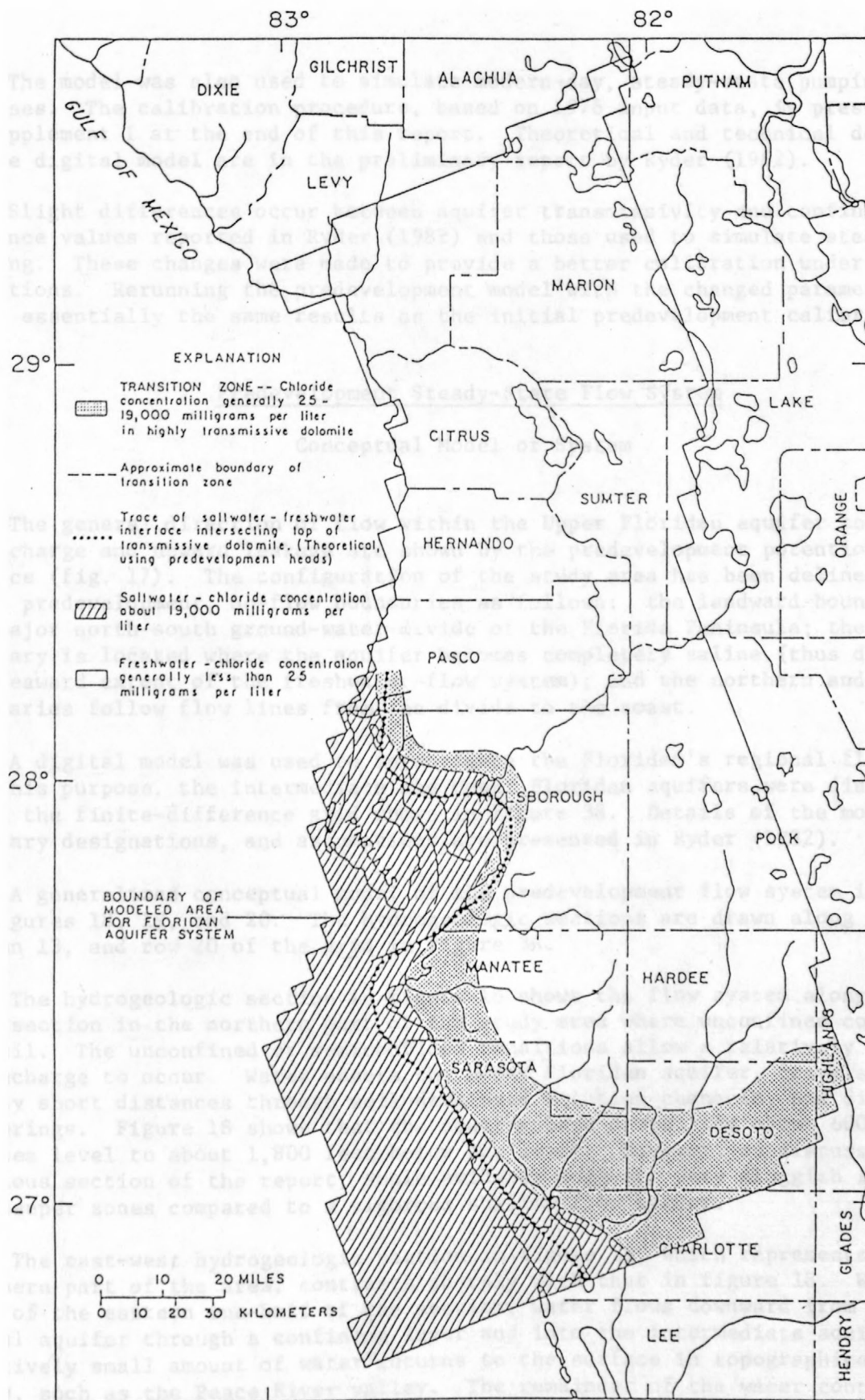
Figure 16.--Saltwater-freshwater transition zone in the highly permeable dolomite of the Upper Floridan aquifer (Hickey, 1981, fig. 15; Wilson, 1982, fig. 7).
