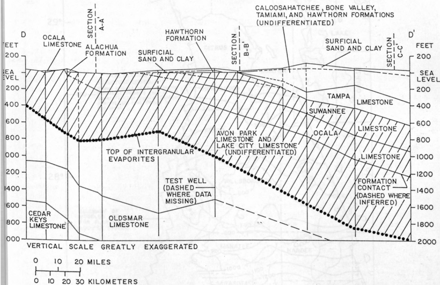
Figure 7.--Geologic section D-D'. (J. A. Miller, written commun., 1981. Shaded area is Upper Floridan aquifer.)
