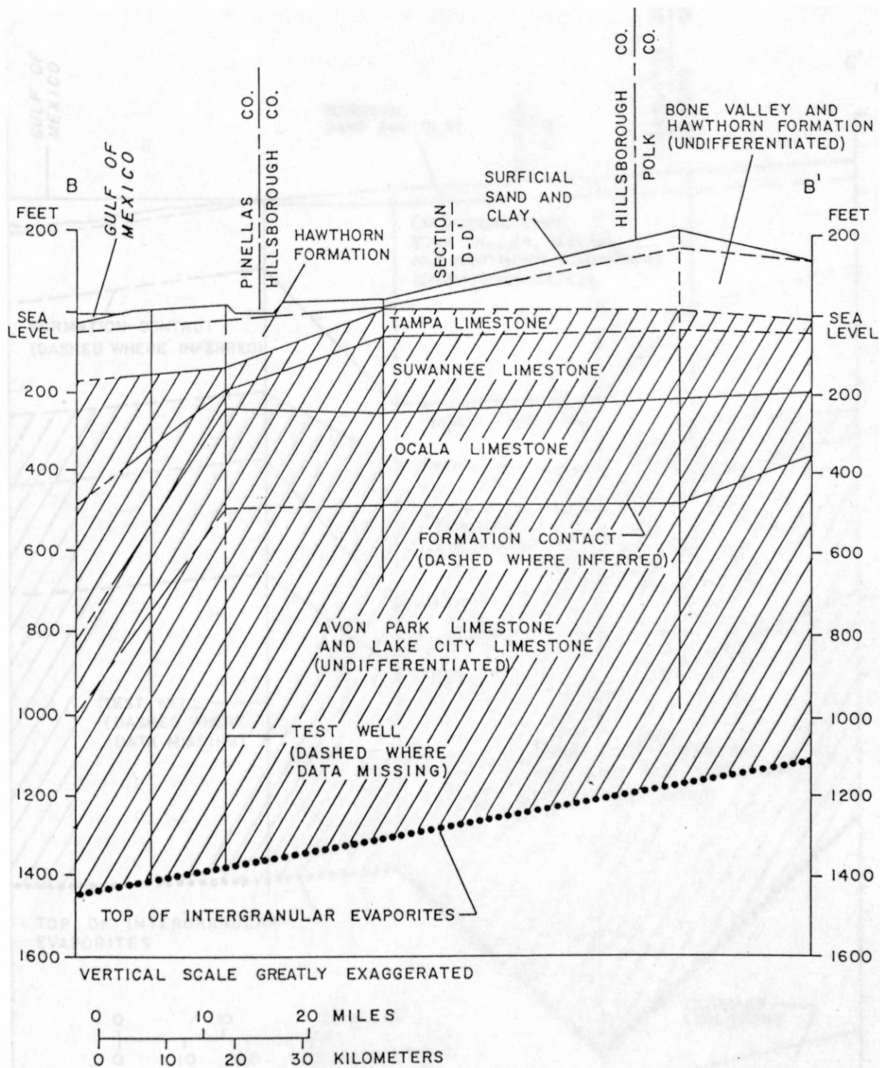
Figure 5.--Geologic section B-B'. (J. A. Miller, written commun., 1981. Shaded area is Upper Floridan aquifer.)
