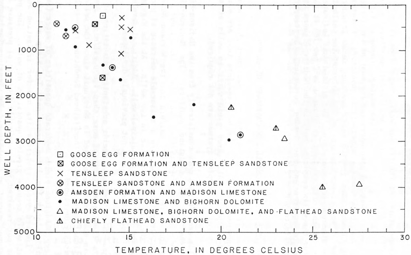
Figure 13.--Well depths and wellhead temperatures.
