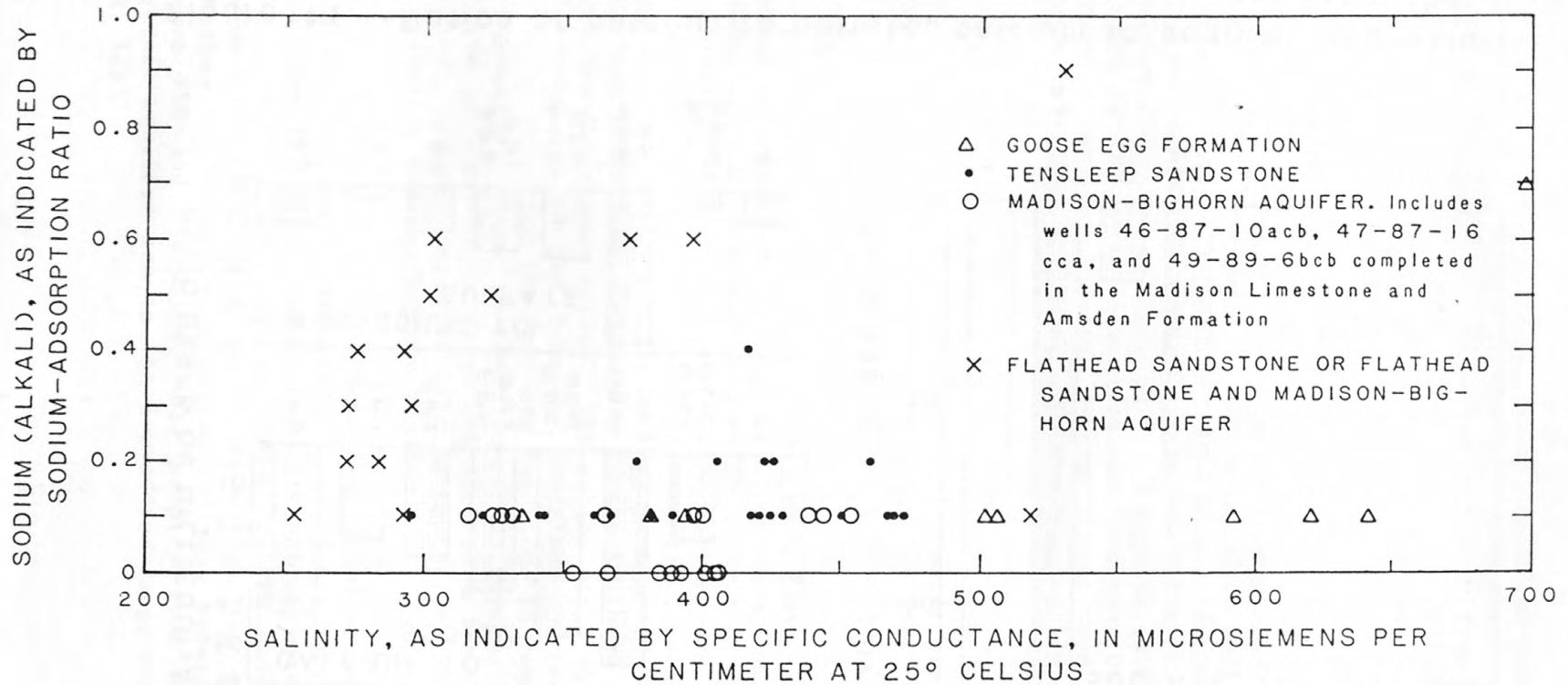
Figure 12.--Comparison of sodium (alkali), as indicated by sodium-adsorption ratio, with salinity, as indicated by specific conductance of water from Paleozoic artesian aquifers.
