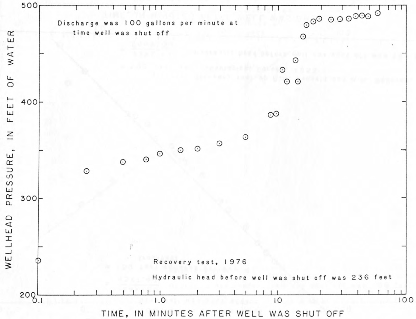
Figure 10.--Recovery curve for the Hyattville town well 49-89-6bcb completed in the Amsden Formation and Madison Limestone.
