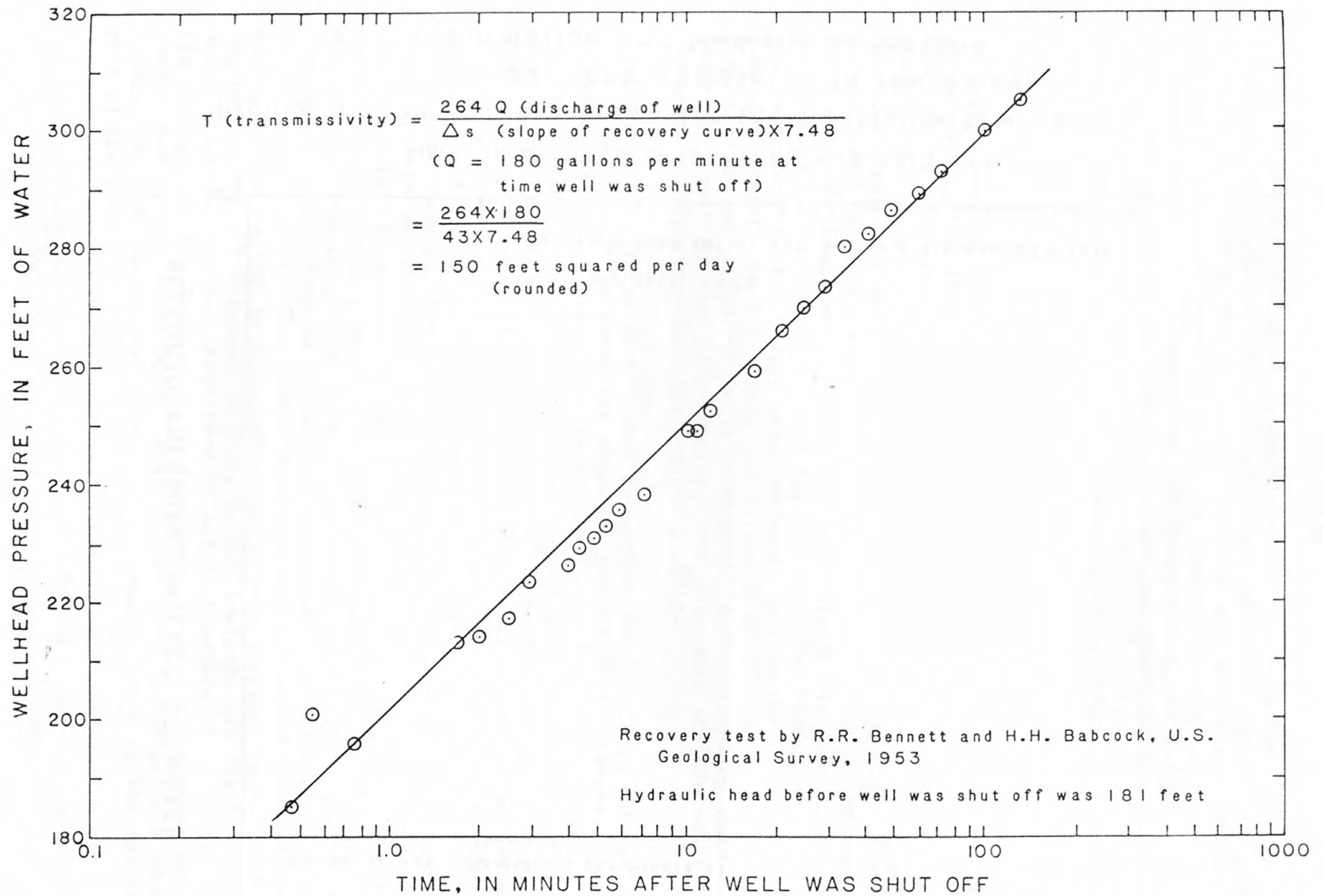
Figure 9.--Recovery curve for well 47-89-13aab completed in the Tensleep Sandstone.
