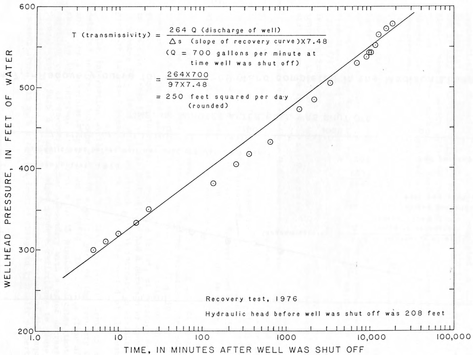
Figure 8.--Recovery curve for well 49-88-29dac completed mainly in the Flathead Sandstone.
