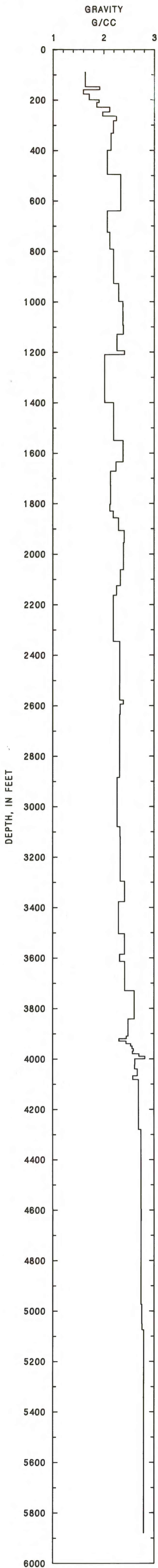
Figure 3.--Plot of interval densities calculated from borehole gravity data in drill hole UE-25p# 1.
