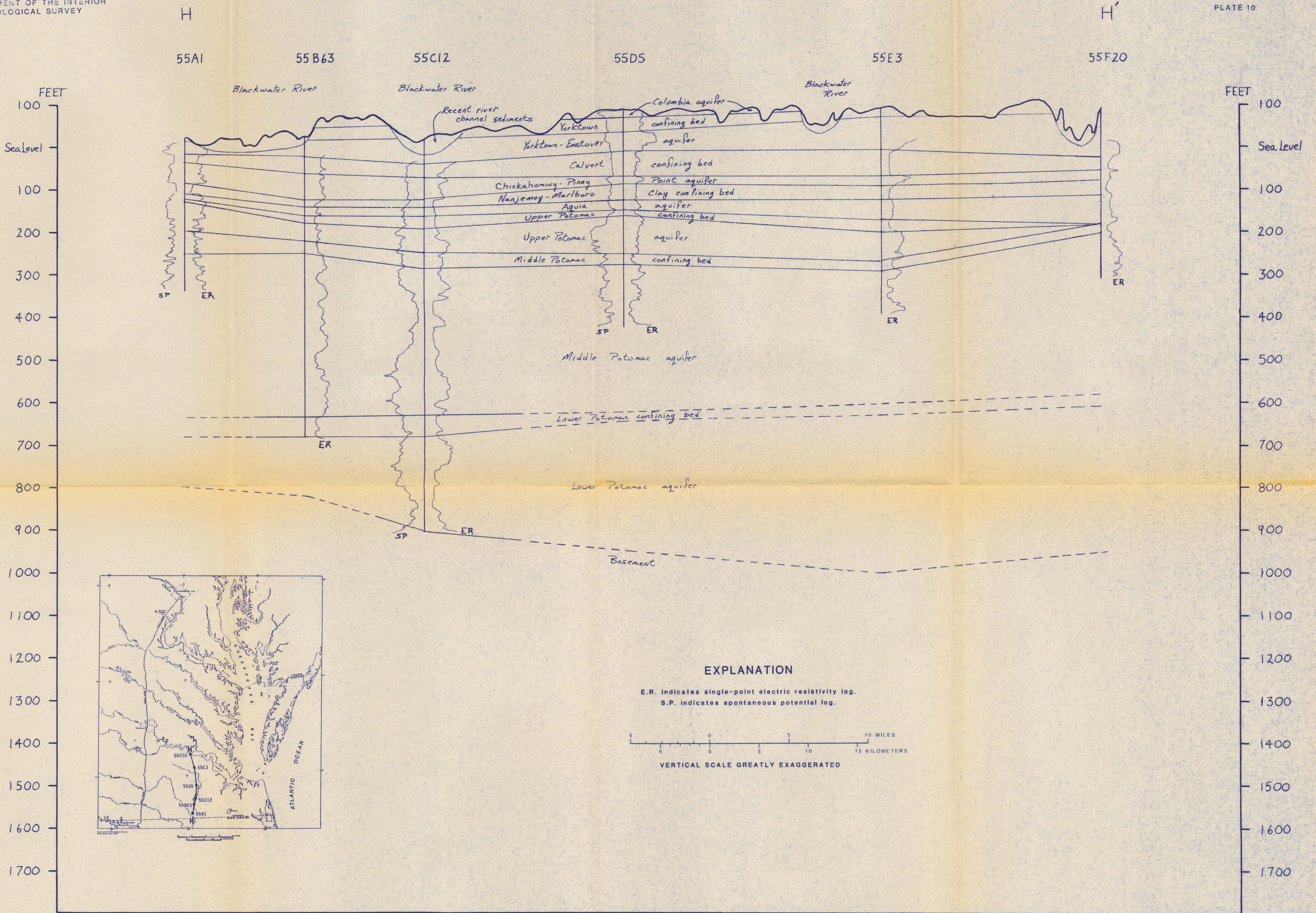
HYDROGEOLOGIC SECTION H-H' FROM WELL 55A1, SOUTHAMPTON COUNTY, TO WELL 55F20, SURRY COUNTY, VIRGINIA.
