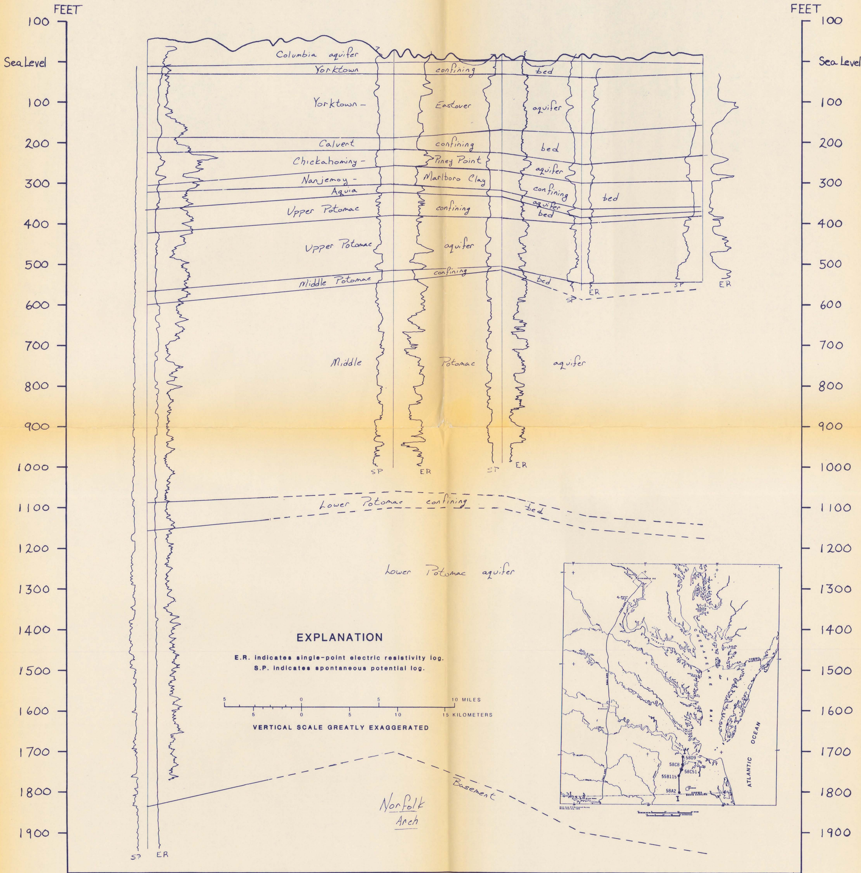
HYDROGEOLOGIC SECTION I-I' FROM WELL 58A2, SUFFOLK, TO WELL 58D9, ISLE OF WIGHT COUNTY, VIRGINIA.
