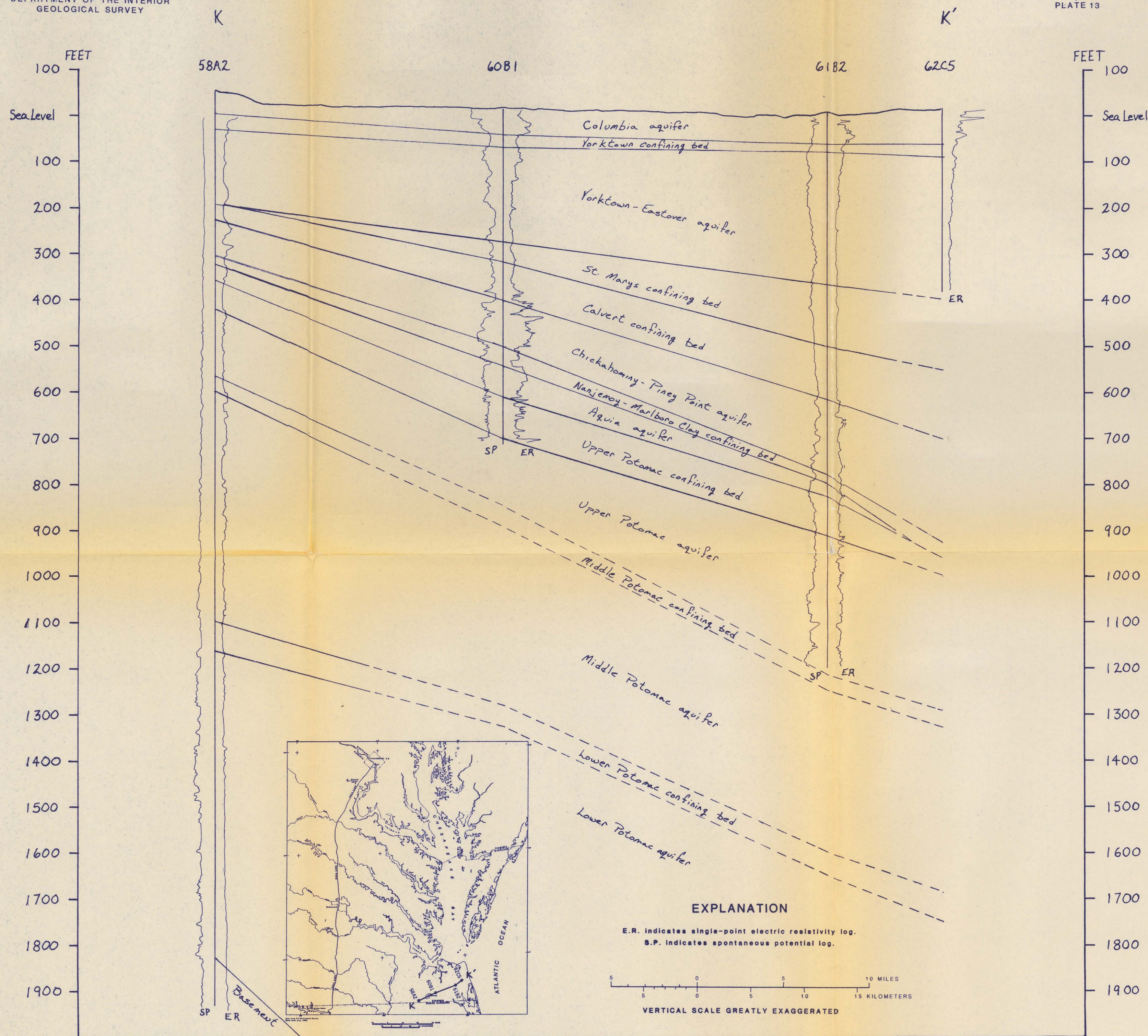
HYDROGEOLOGIC SECTION K-K' FROM WELL 58A2, SUFFOLK, TO WELL 62C5, VIRGINIA BEACH, VIRGINIA.
